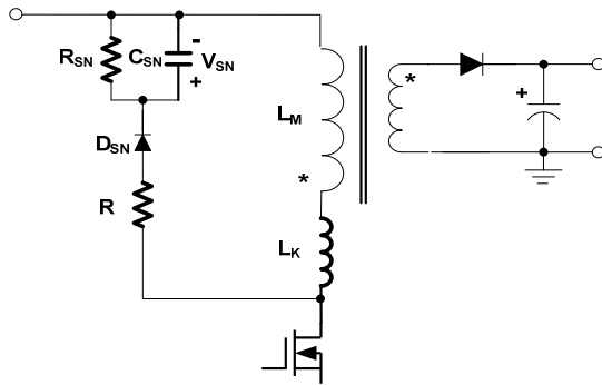
Figure 14: RCD Snubber
