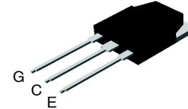
TO-3P-3LD / EIAJ SC-65, ISOLATED CASE 340BZ
