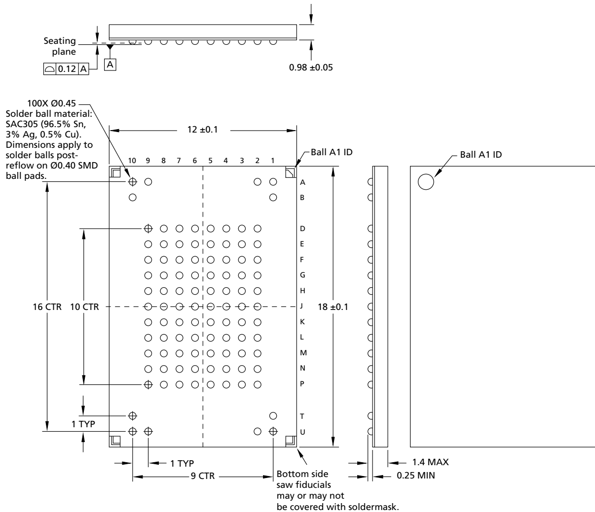
Figure 9: 100-Ball LBGAs – 12mm x 18mm (Package Code: H3)
