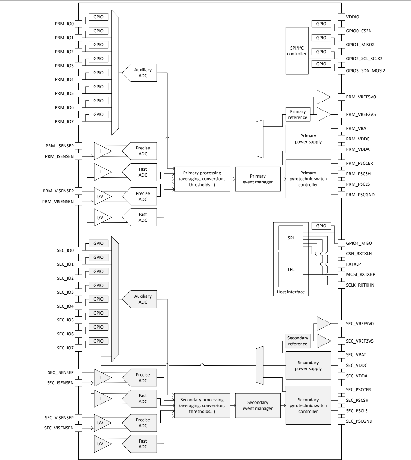
Figure 1. Block diagram
