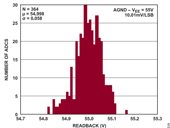
Figure 14. V_{EE} Readback
