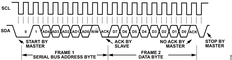
Figure 33. Reading the Interrupt Register (Short Form)
