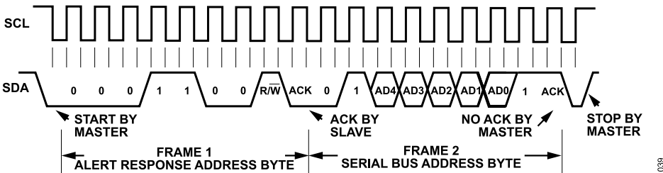
Figure 34. Reading from Alert Response Address
