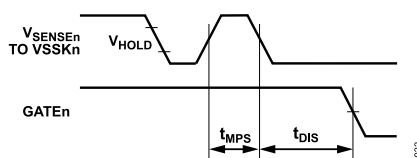
Figure 28. DC Disconnect Timing
