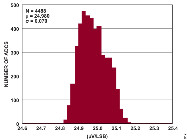
Figure 12. Port Current Readback LSB
