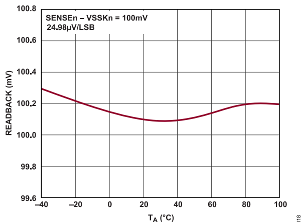
Figure 13. Port Current Readback vs. Temperature
