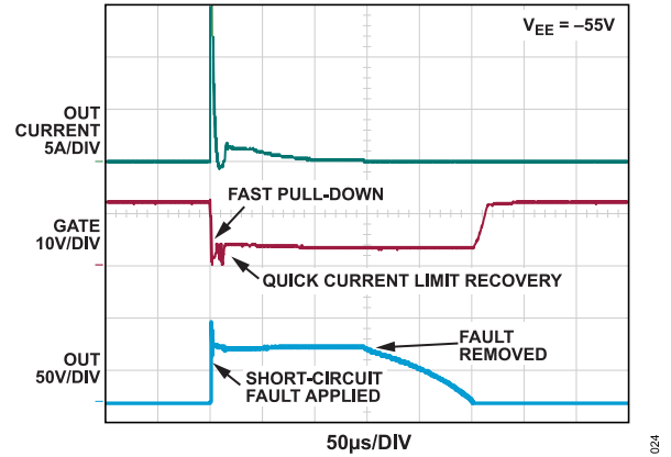
Figure 19. Short-Circuit Recovery
