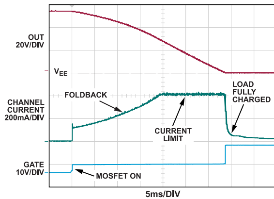
Figure 18. Powering Up into 180µF
