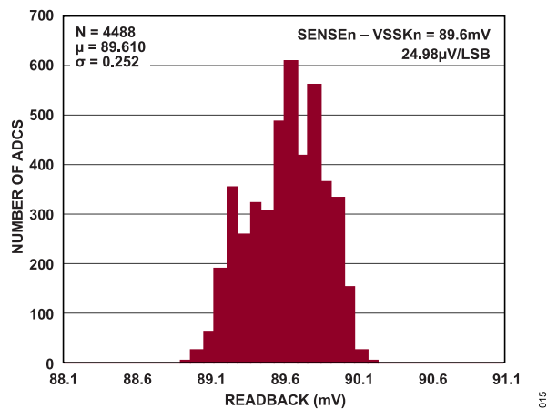
Figure 10. Port Current Readback
