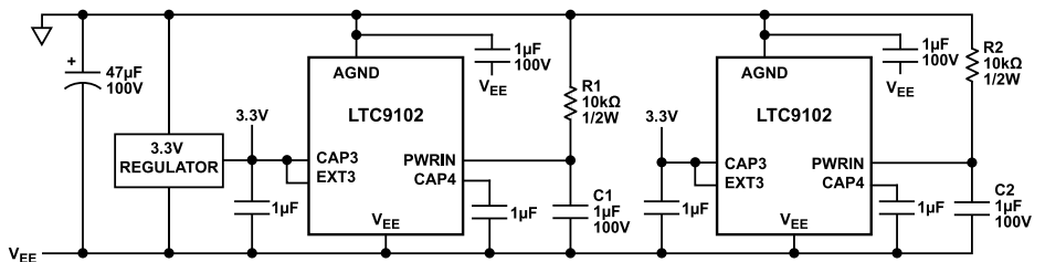
Figure 42. Power Supply Configuration with External 3.3V Regulator
