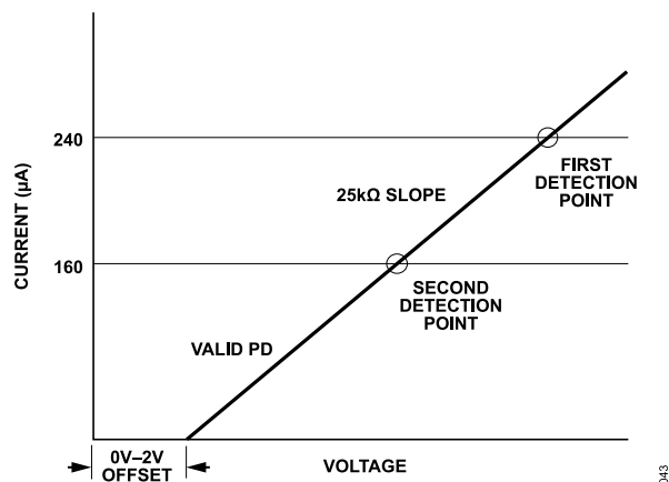
Figure 37. PD Detection
