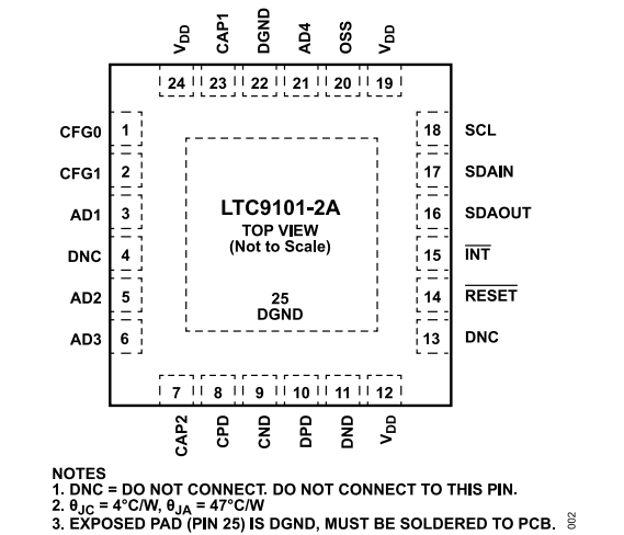
Figure 2. LTC9101-2A
