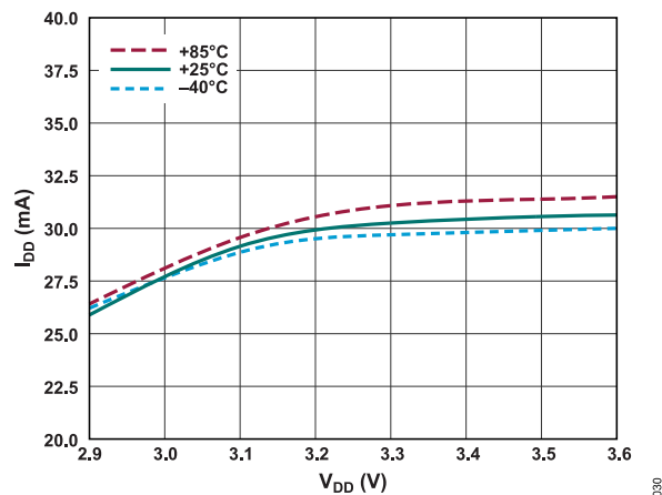
Figure 25. V_{DD} Supply Current vs. Voltage and Temperature
