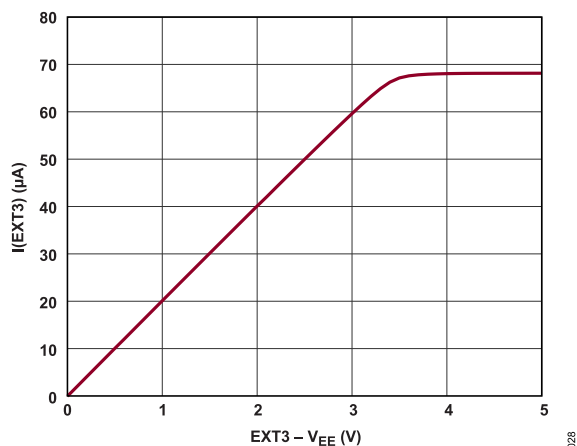
Figure 23. EXT3 Pin Current vs. Voltage
