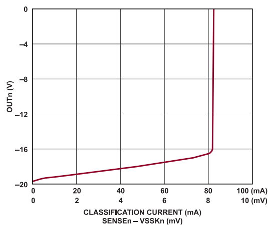
Figure 9. Classification Current Compliance
