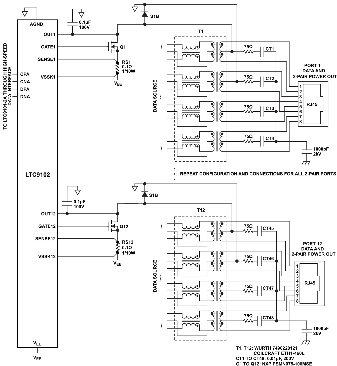
Figure 47. Alternative A (MDI-X) and B(S), 2-Pair, 1000BASE-T, IEEE 802.3at, Type 2 PSE, Ports 1 and 12 Shown
