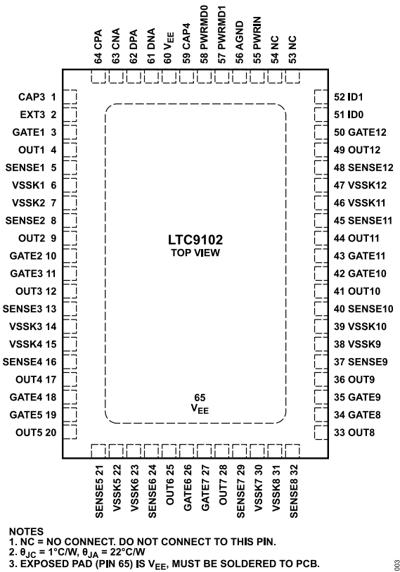
Figure 3. LTC9102
