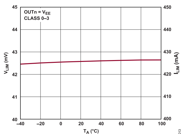
Figure 8. I_{LIM} vs. Temperature
