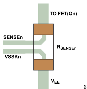
Figure 46. R_{SENSE} Kelvin Connections
