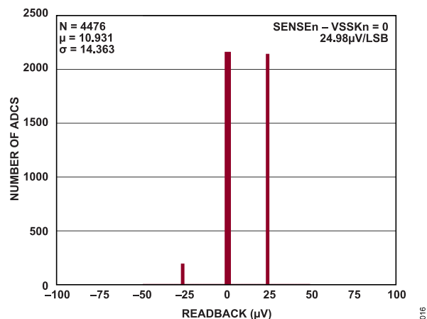
Figure 11. Port Current Readback Offset
