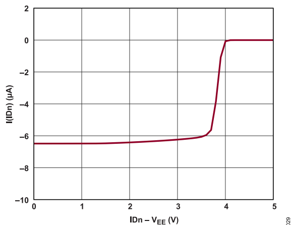
Figure 24. IDn Pin Current vs. Voltage
