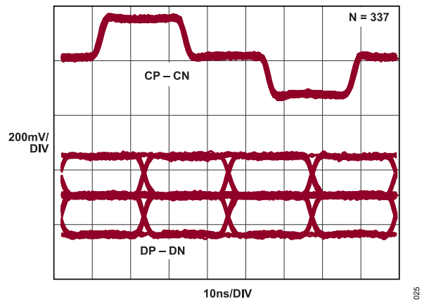
Figure 20. Clock and Data Write Eye Diagram
