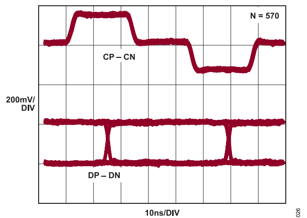
Figure 21. Clock and Data Read Eye Diagram
