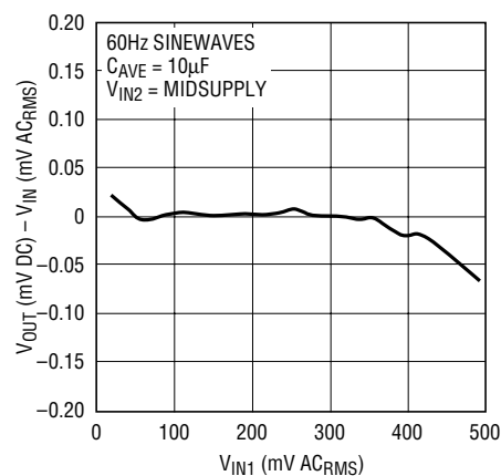
AC Linearity
