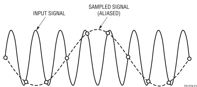
Figure 17. Time Domain View of Aliasing
