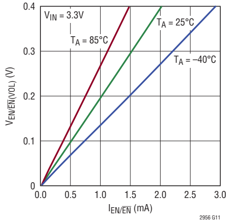
EN/ \overline{\text{EN}} Output Low Voltage vs Current
