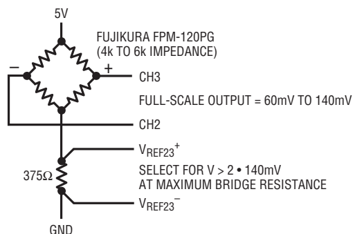
(19b) Full-Bridge, Current Sense
