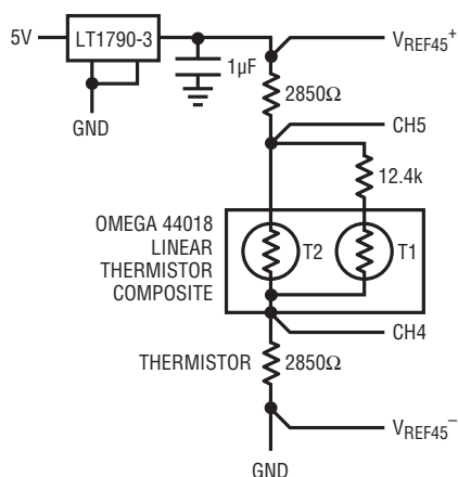
(19c) Half-Bridge, Voltage Sense
