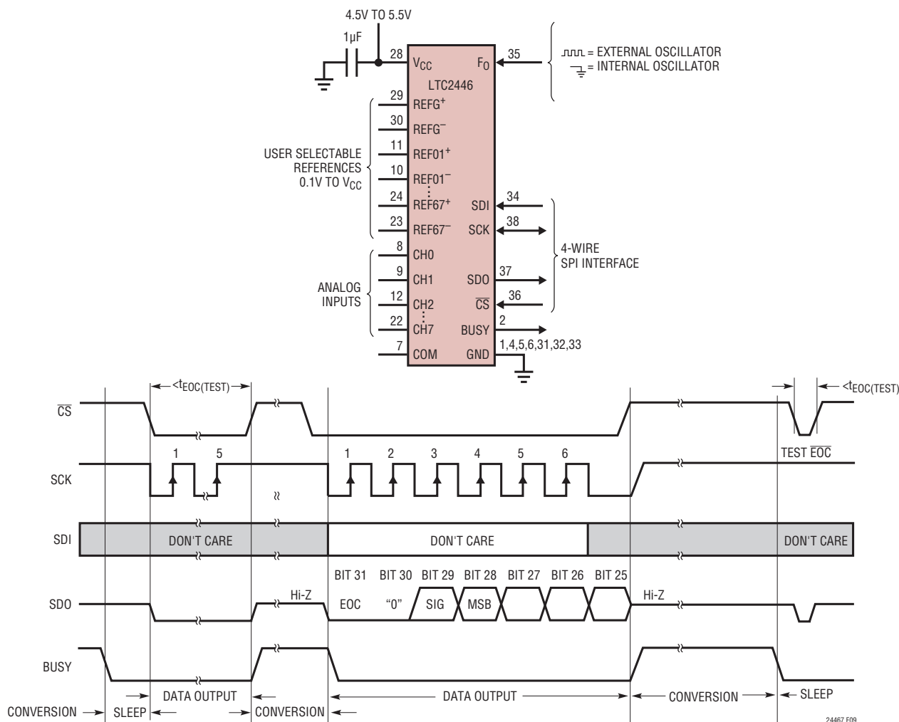
Figure 9. Internal Serial Clock, Reduced Data Output Length
