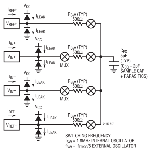
Figure 17. LTC2446 Input Structure
