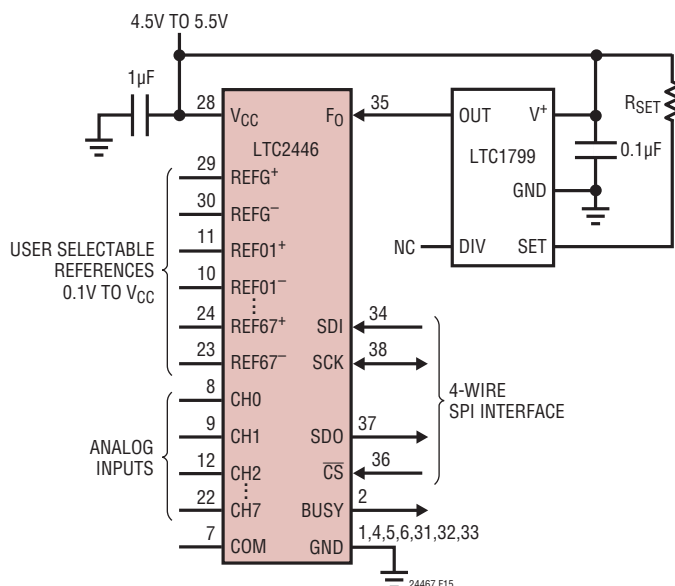
Figure 15. Simple External Clock Source
