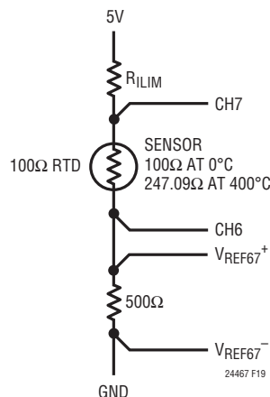
(19d) Half-Bridge, Current Sense
