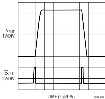
Large-Signal Settling—Fast Mode
