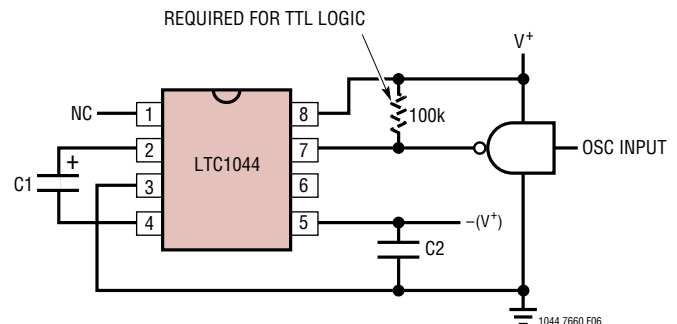
Figure 6. External Clocking
