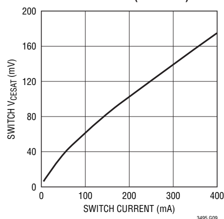
SW Saturation Voltage vs Switch Current (LT3495-1)
