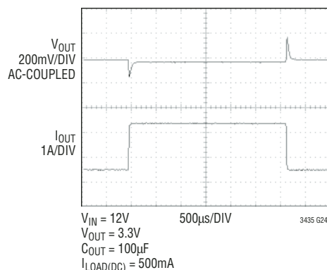
Step Response
