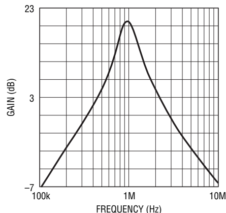
Frequency Response Plot of Bandpass Filter
