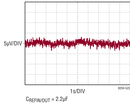
Internal 2.048V REFIN/OUT Low Frequency 0.1Hz to 10Hz Noise
