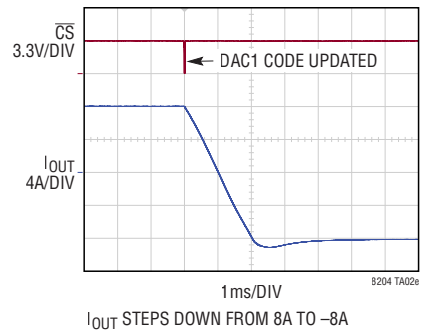
I_{OUT} Commanded to Step Down
