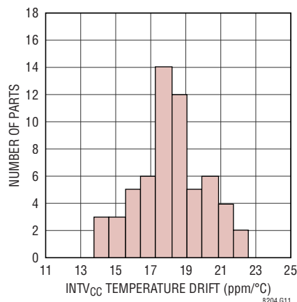
INTV CC Temperature Drift Distribution
