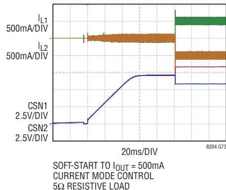
Soft Start-Up Waveforms (H-Bridge Configuration)
