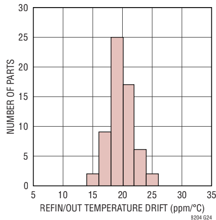
Internal 2.048V REFIN/OUT Temperature Drift Distribution
