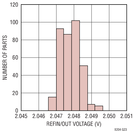
Internal 2.048V REFIN/OUT Voltage Distribution
