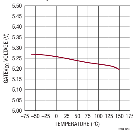
GATEV CC Voltage vs Temperature
