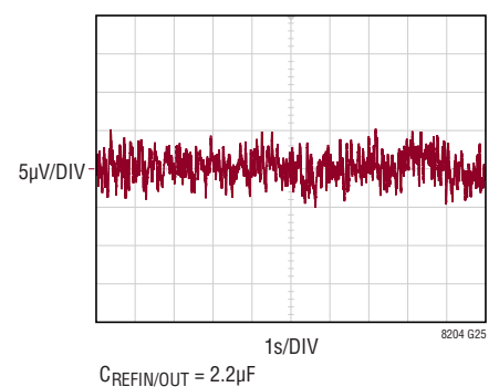
Internal 4.096V REFIN/OUT Low Frequency 0.1Hz to 10Hz Noise
