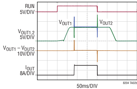
Soft Start Up and Shutdown with I_{OUT} = 8A
