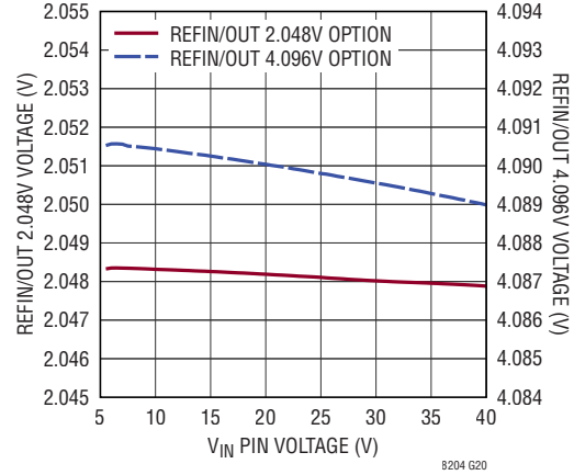
Internal REFIN/OUT Voltage vs V IN
