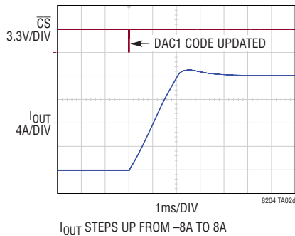
I_{OUT} Commanded to Step Up
