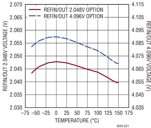
Internal REFIN/OUT Voltage vs Temperature
