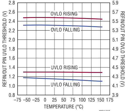
REFIN/OUT Pin Threshold External REFIN/OUT Option
