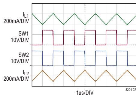
Switching Waveforms (H-Bridge Configuration)
