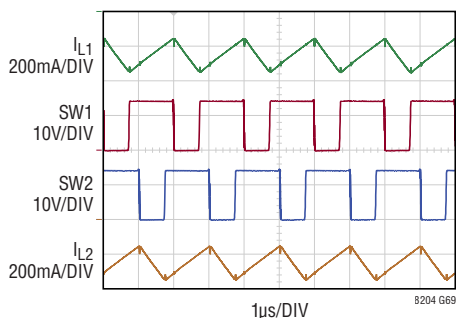
Switching Waveforms (Half-Bridge Configuration)
