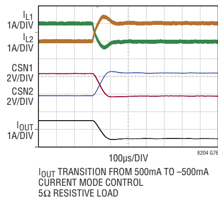
I_{OUT} Step Response to DAC (H-Bridge Configuration)
