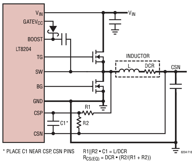
Figure 18. Using the Inductor DCR to Sense Current with the LT8204
