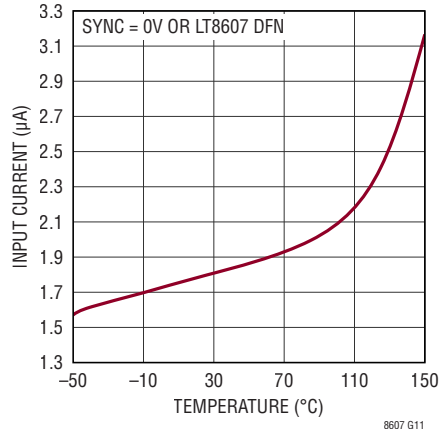
No Load Supply Current vs Temperature (Not Switching)
