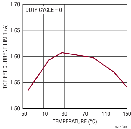
Top MOSFET Current Limit vs Temperature
