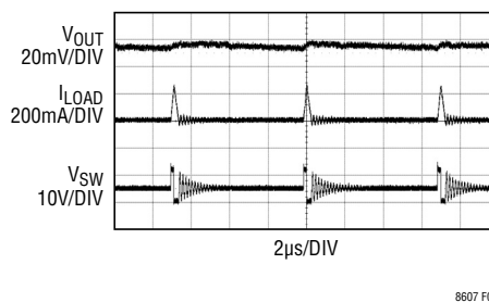
Figure 3. Burst Mode Operation
