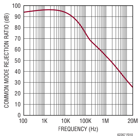
Figure 10. LTC6227-LT5401 Based Instrumentation Amplifier CMRR
