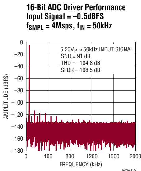
Figure 5. Measured Performance of LTC6227 Based Driver Driving the AD7380
