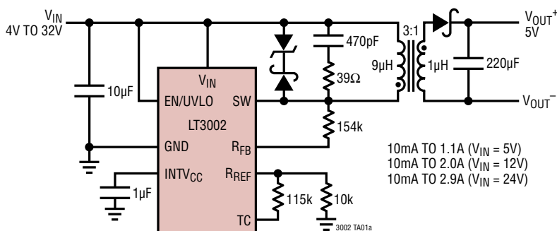
4V to 32V IN /5V OUT Isolated Flyback Converter
