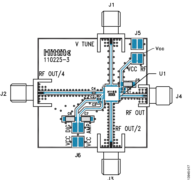
Figure 17. Evaluation PCB
