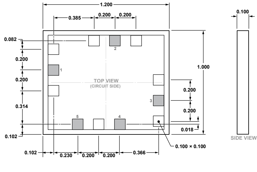
Figure 28. 5-Pad Bare Die [CHIP] (C-5-5) Dimensions shown in millimeters
