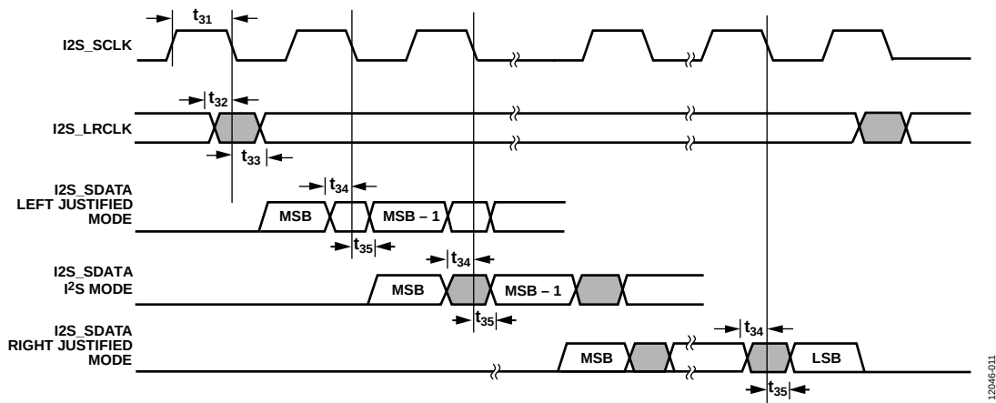
Figure 11. I 2 S Timing
