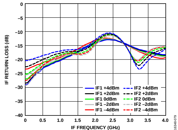
Figure 79. IF Return Loss vs. IF Frequency over LO Powers, LO Frequency = 7 GHz, T_A = 25^\circ\text{C}
