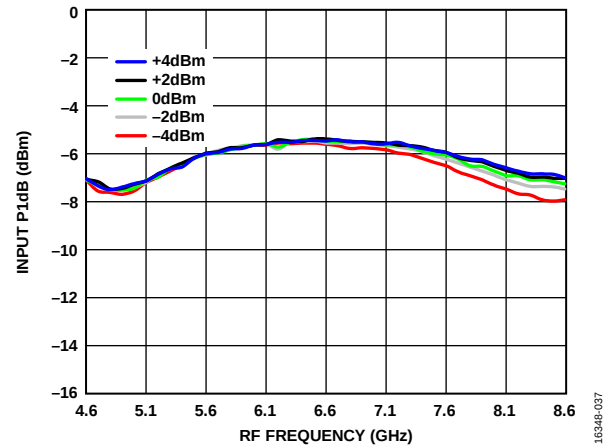
Figure 37. Input P1dB vs. RF Frequency over LO Powers, T_A = 25^\circ\text{C}
