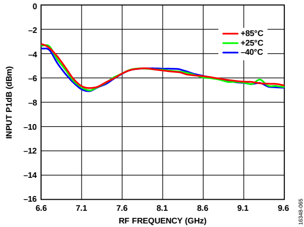
Figure 65. Input P1dB vs. RF Frequency over Temperatures, LO Power = 0 dBm
