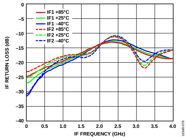
Figure 78. IF Return Loss vs. IF Frequency over Temperatures, LO Frequency = 7 GHz, LO Power = 0 dBm
