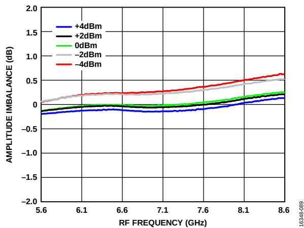
Figure 89. Amplitude Imbalance vs. RF Frequency over LO Powers, IF = 1000 MHz, T_A = 25^\circ\text{C} , Lower Sideband
