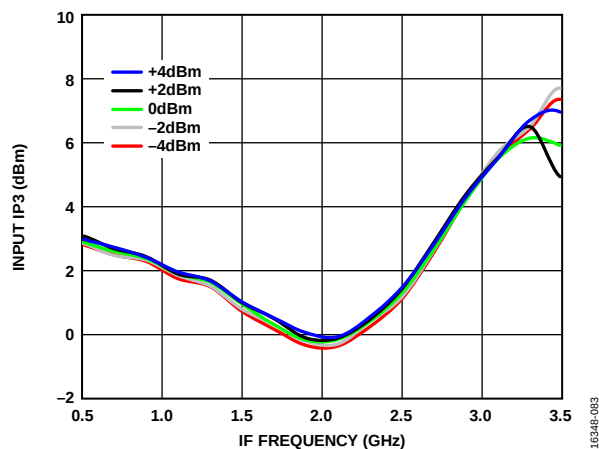
Figure 83. Input IP3 vs. IF Frequency over LO Powers, LO Frequency = 7 GHz, T_A = 25^\circ\text{C}
