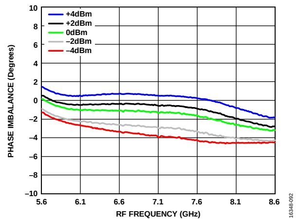
Figure 92. Phase Imbalance vs. RF Frequency over LO Powers, IF = 1000 MHz, T_A = 25^\circ\text{C} , Lower Sideband
