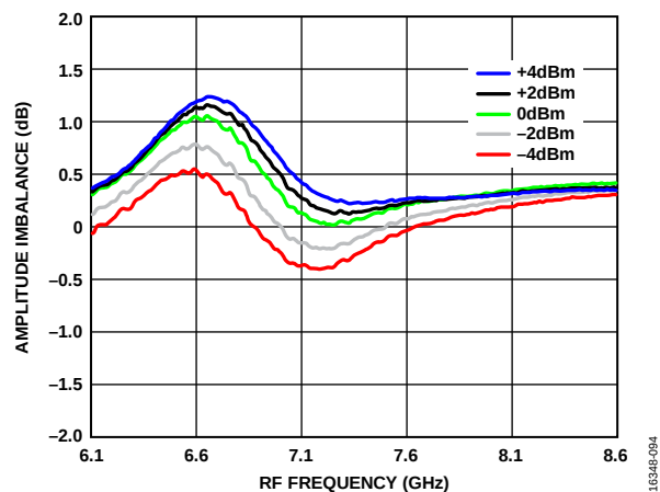
Figure 94. Amplitude Imbalance vs. RF Frequency over LO Powers, IF = 1000 MHz, T_A = 25^\circ\text{C} , Upper Sideband
