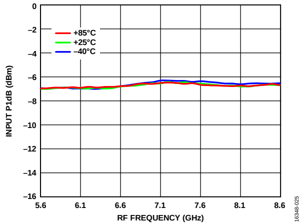
Figure 25. Input P1dB vs. RF Frequency over Temperatures, LO Power = 0 dBm
