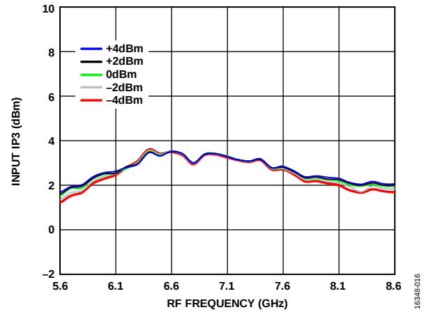
Figure 16. Input IP3 vs. RF Frequency over LO Powers, T_A = 25^\circ\text{C}
