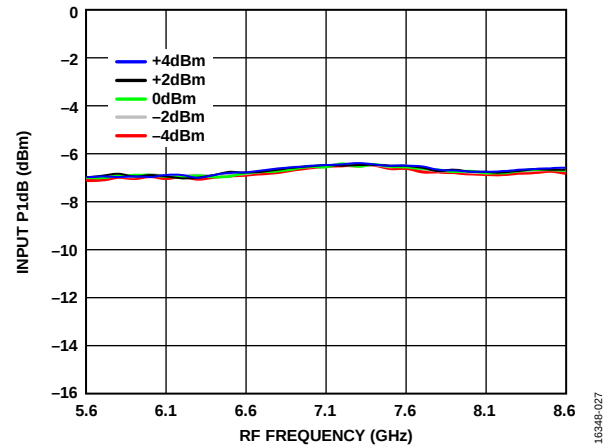
Figure 27. Input P1dB vs. RF Frequency over LO Powers, T_A = 25^\circ\text{C}
