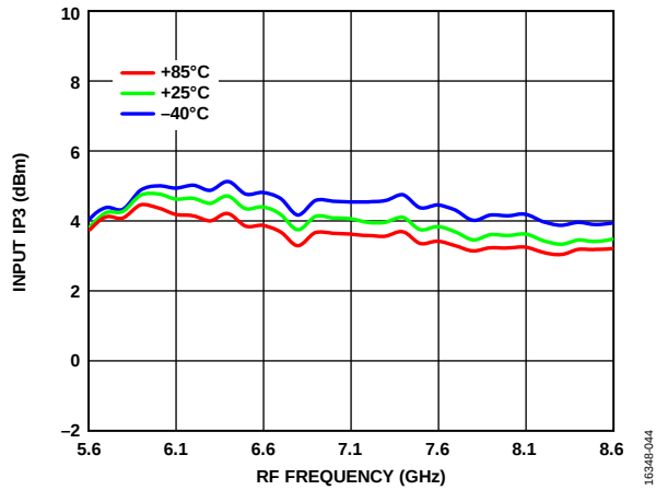
Figure 44. Input IP3 vs. RF Frequency over Temperatures, LO Power = 0 dBm
