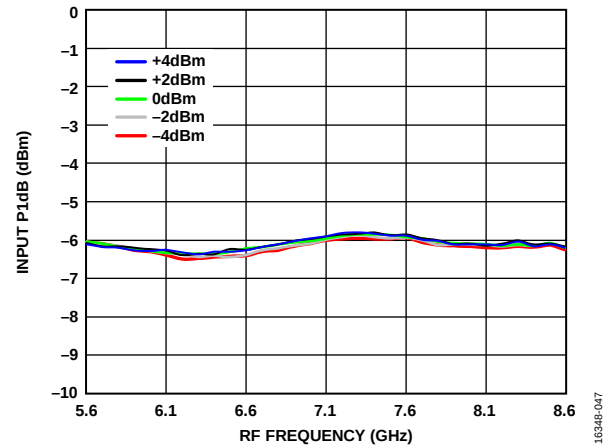
Figure 47. Input P1dB vs. RF Frequency over LO Powers, T_A = 25^\circ\text{C}
