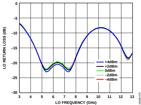
Figure 75. LO Return Loss vs. LO Frequency over LO Powers, T_A = 25^\circ\text{C}
