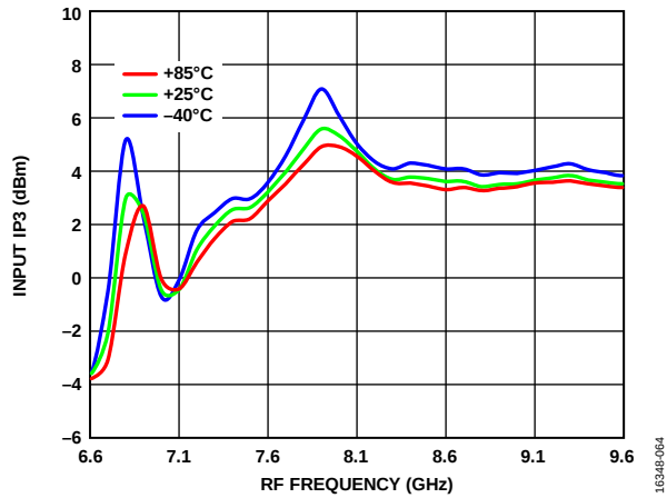
Figure 64. Input IP3 vs. RF Frequency over Temperatures, LO Power = 0 dBm
