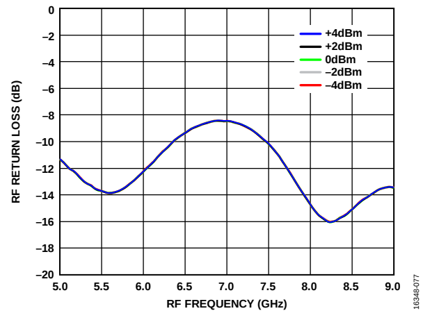
Figure 77. RF Return Loss vs. RF Frequency over LO Powers, LO Frequency = 7 GHz, T_A = 25^\circ\text{C}
