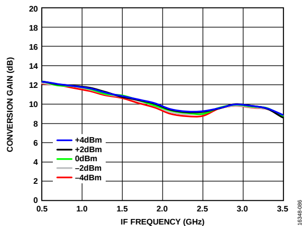
Figure 86. Conversion Gain vs. IF Frequency over LO Powers, LO Frequency = 7 GHz, T_A = 25^\circ\text{C}
