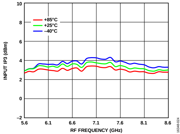
Figure 24. Input IP3 vs. RF Frequency over Temperatures, LO Power = 0 dBm
