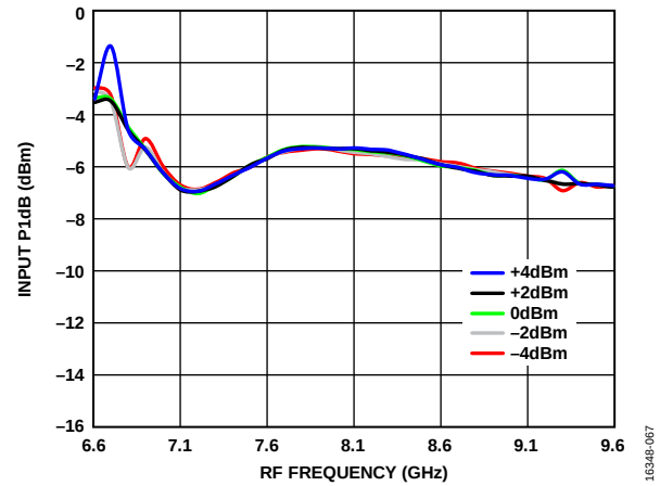
Figure 67. Input P1dB vs. RF Frequency over LO Powers, T_A = 25^\circ\text{C}
