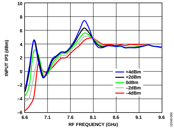
Figure 66. Input IP3 vs. RF Frequency over LO Powers, T_A = 25^\circ\text{C}
