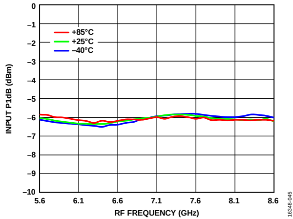
Figure 45. Input P1dB vs. RF Frequency over Temperatures, LO Power = 0 dBm
