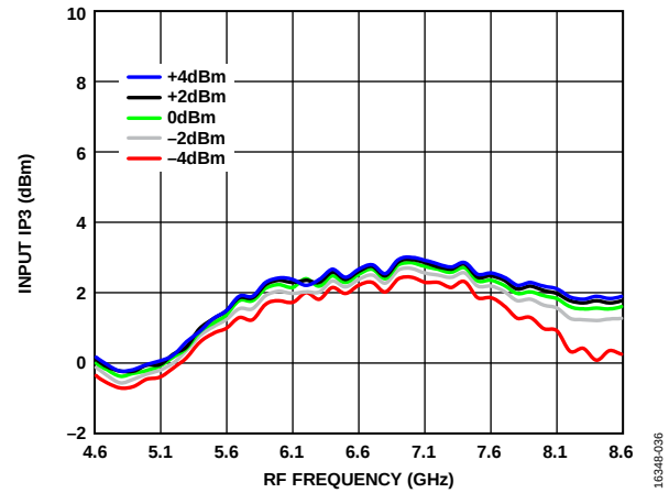
Figure 36. Input IP3 vs. RF Frequency over LO Powers, T_A = 25^\circ\text{C}
