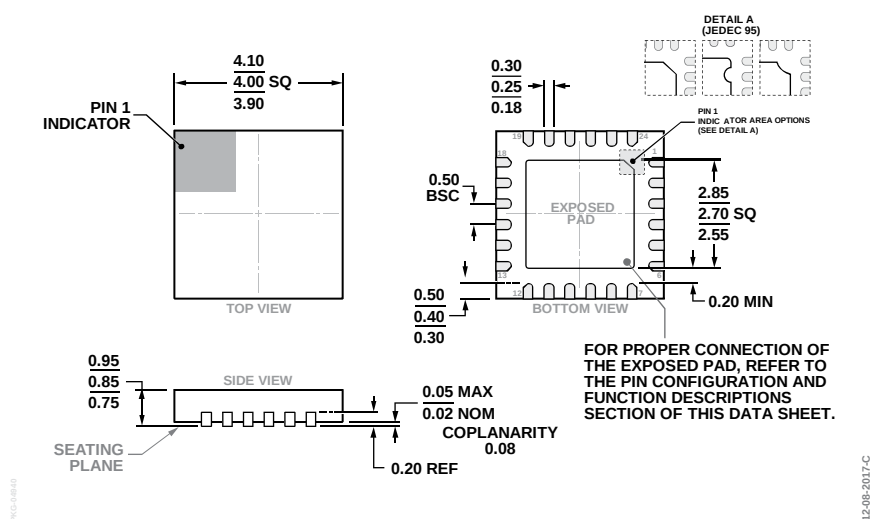
Figure 101. 24-Lead Lead Frame Chip Scale Package [LFCSP], 4 mm x 4 mm Body and 0.85 mm Package Height (HCP-24-3)
