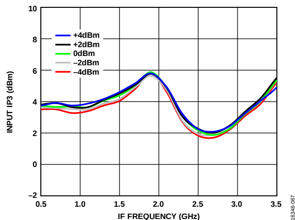
Figure 87. Input IP3 vs. IF Frequency over LO Powers, LO Frequency = 7 GHz, T_A = 25^\circ\text{C}
