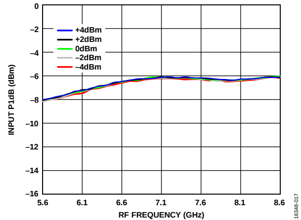
Figure 17. Input P1dB vs. RF Frequency over LO Powers, T_A = 25^\circ\text{C}
