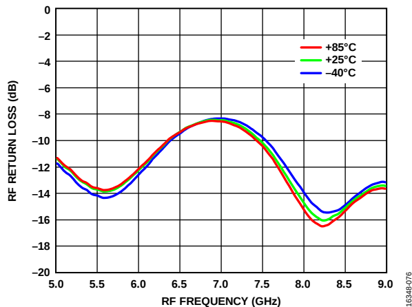
Figure 76. RF Return Loss vs. RF Frequency over Temperatures, LO Frequency = 7 GHz, LO Power = 0 dBm
