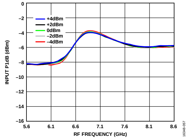
Figure 57. Input P1dB vs. RF Frequency over LO Powers, T_A = 25^\circ\text{C}
