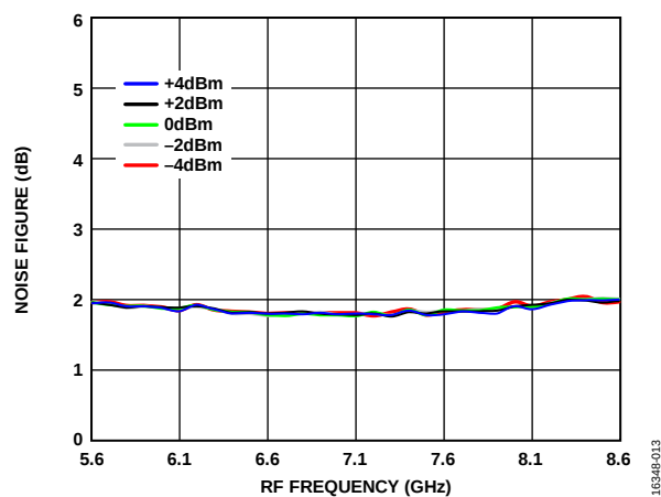
Figure 13. Noise Figure vs. RF Frequency over LO Powers, T_A = 25^\circ\text{C}
