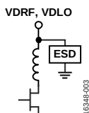
Figure 3. VDRF, VDLO Interface
