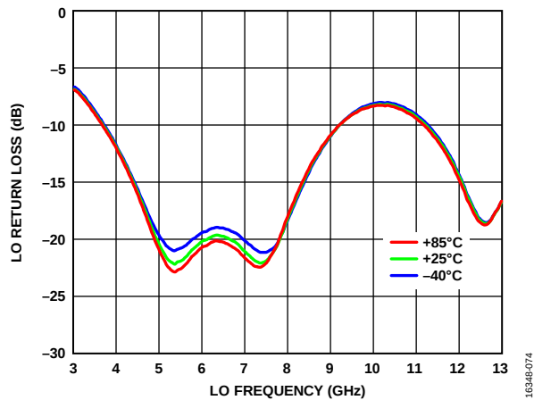
Figure 74. LO Return Loss vs. LO Frequency over Temperatures, LO Power = 0 dBm
