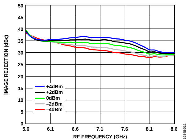
Figure 12. Image Rejection vs. RF Frequency over LO Powers, T_A = 25^\circ\text{C}
