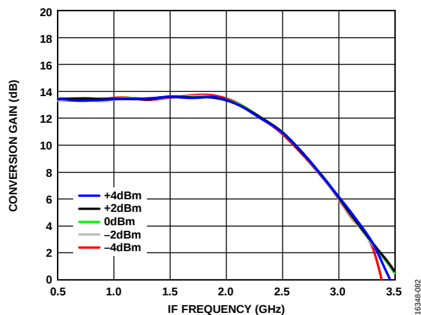
Figure 82. Conversion Gain vs. IF Frequency over LO Powers, LO Frequency = 7 GHz, T_A = 25^\circ\text{C}
