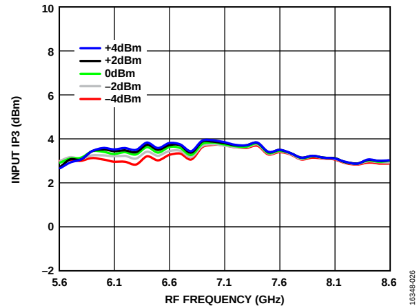
Figure 26. Input IP3 vs. RF Frequency over LO Powers, T_A = 25^\circ\text{C}
