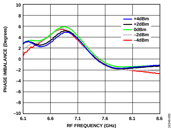
Figure 95. Phase Imbalance vs. RF Frequency over LO Powers, IF = 1000 MHz, T_A = 25^\circ\text{C} , Upper Sideband
