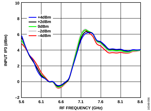
Figure 56. Input IP3 vs. RF Frequency over LO Powers, T_A = 25^\circ\text{C}
