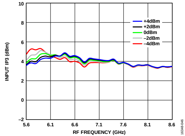
Figure 46. Input IP3 vs. RF Frequency over LO Powers, T_A = 25^\circ\text{C}
