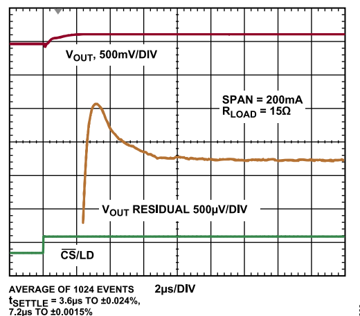
Figure 10. Settling 145 mA to 155 mA Step (VOUT Is the Output Voltage)
