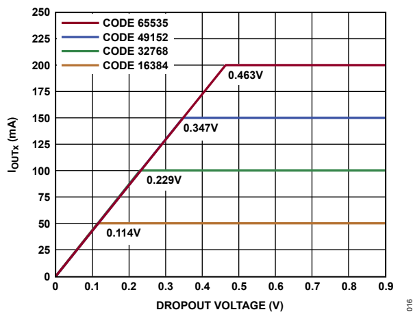
Figure 20. I_{OUTx} vs. Dropout Voltage for Multiple Codes (200 mA Span)
