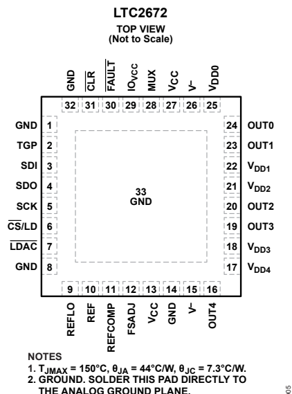
Figure 5. LFCSP Pin Configuration
