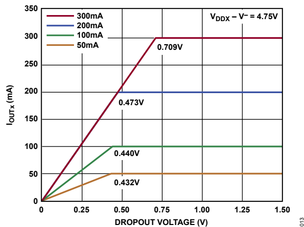
Figure 16. I_{OUTX} vs. Dropout Voltage for Multiple Current Ranges
