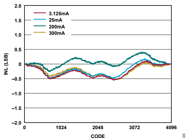
Figure 8. LTC2672-12 INL
