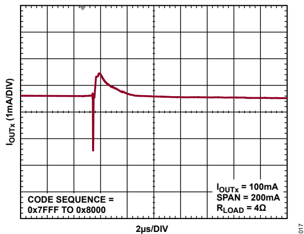
Figure 21. Midscale Glitch
