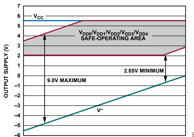
Figure 33. Output Supply Safe Operating Area
