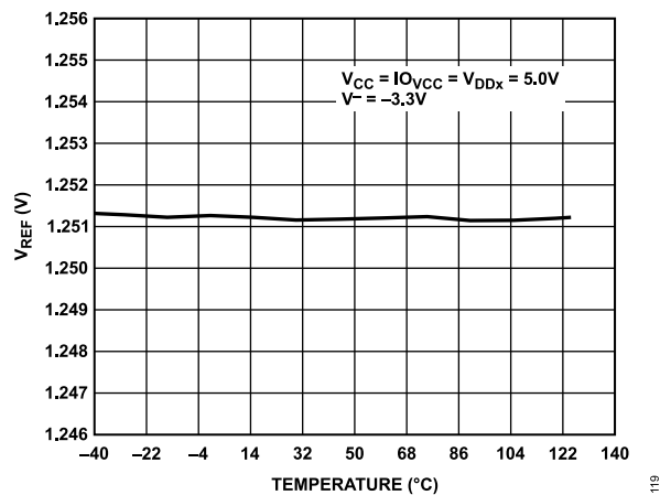
Figure 19. V_{REF} vs. Temperature (WLCSP)
