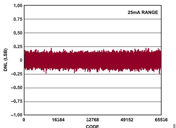
Figure 11. LTC2672-16 DNL
