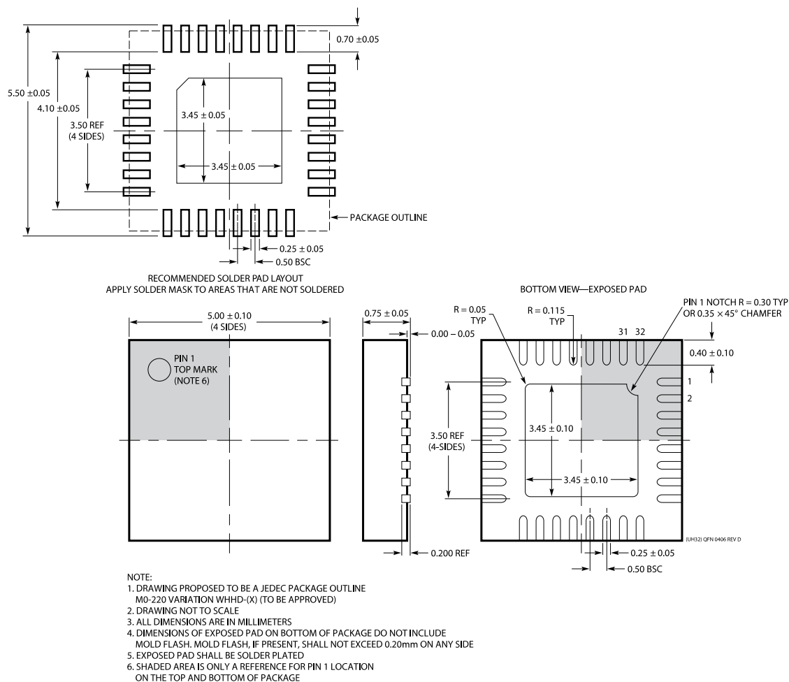
Figure 36. 32-Lead Plastic QFN 5 mm × 5 mm Body (Reference LTC DWG # 05-08-1693 Rev. D)
