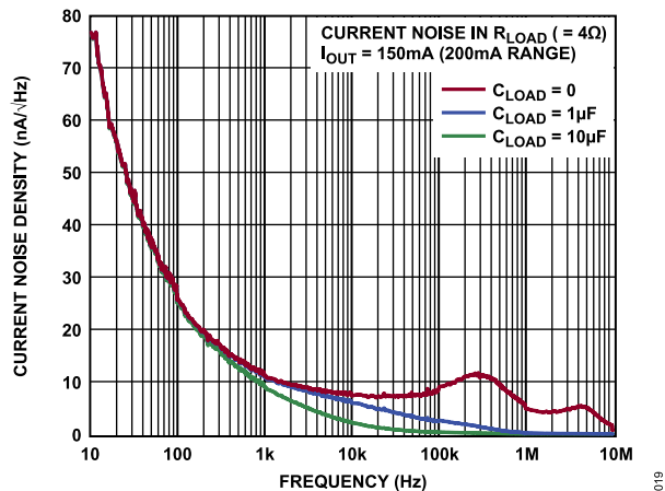
Figure 22. Current Noise Density vs. Frequency, Grounded C_{LOAD} = 0\mu F , 1\mu F , and 10\mu F
