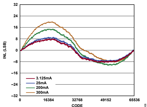
Figure 7. LTC2672-16 INL
