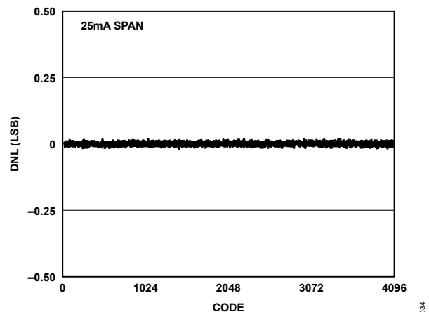
Figure 12. LTC2672-12 DNL
