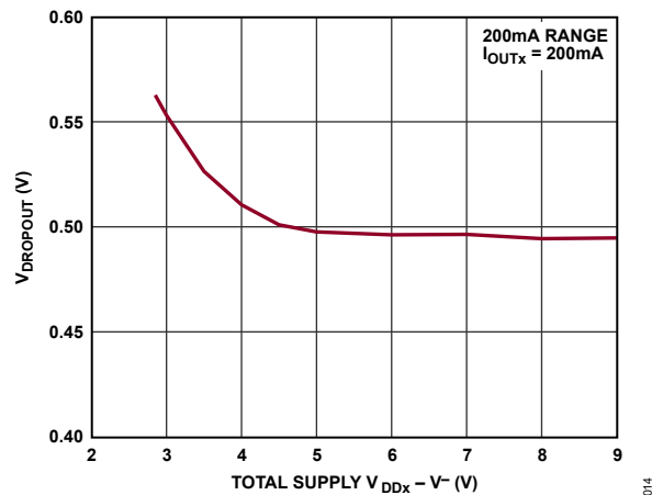
Figure 17. V_{DROP} vs. Total Supply V_{DD} - V^-
