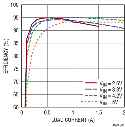
3.3V OUT Efficiency, 1MHz, CCM
