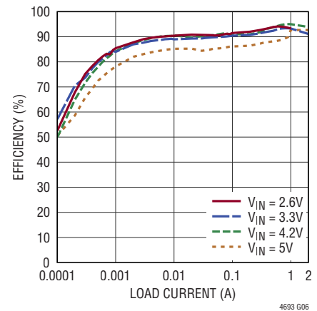
3.3V OUT Efficiency, 1MHz, Burst Mode Operation
