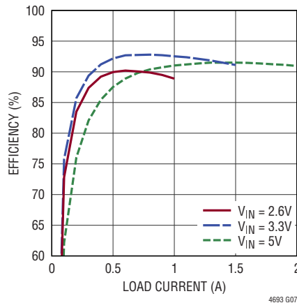
5V OUT Efficiency, 1MHz, CCM
