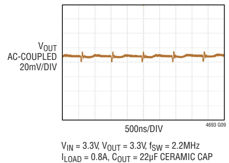
Output Ripple
