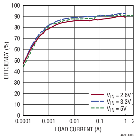
5V OUT Efficiency, 1MHz, Burst Mode Operation
