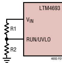
Figure 1. Circuit to Set V IN UVLO
