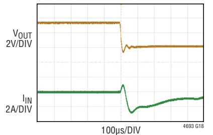
Short-Circuit with 2A Load
