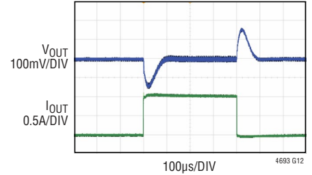
Load Transient Response 3.3V IN to 3.3V OUT
