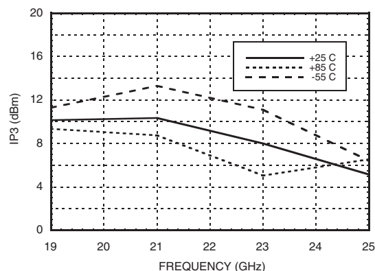
Input IP3 vs. Temperature @ LO = -5 dBm, Vdd = +3V *
