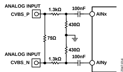
Figure 12. Typical Pseudo Differential Input Resistor Divider Network
