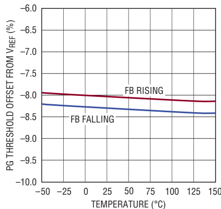
PG Thresholds Below V_{\text{REF}}
