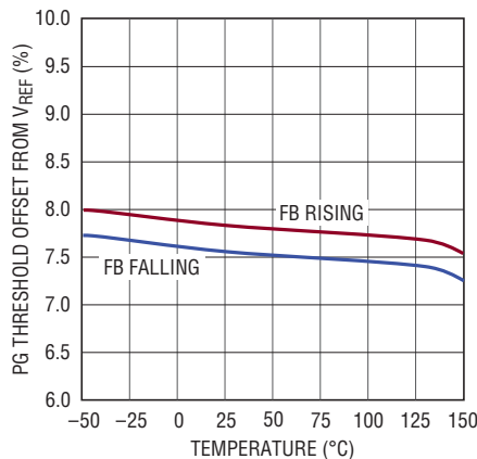
PG Thresholds Above V_{\text{REF}}
