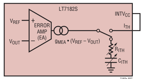
Figure 7. Programmable Internal Compensation
