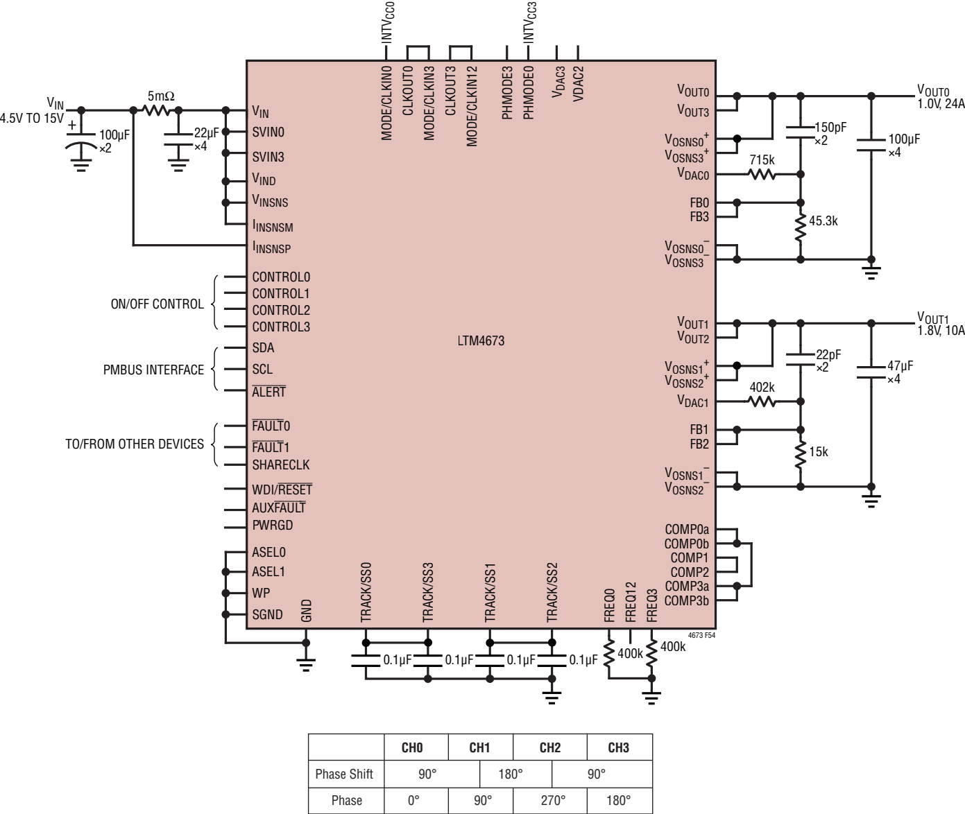
Figure 54. Parallel Operation with 1MHz Clock and Interleaved Phases
