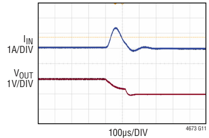
Short-Circuit Waveform with No Load Current Exist, V_{OUT} Undervoltage Fault Response
