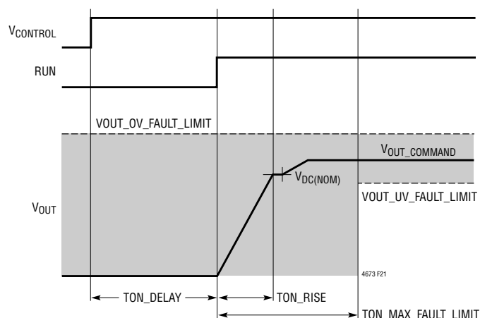
Figure 21. Typical ON Sequence Using Control Pin
