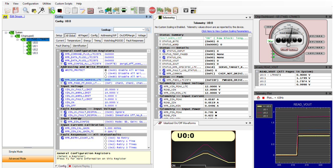
Figure 36. LTpowerPlay Snapshot
