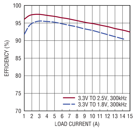
Figure 24. Efficiency, 3.3VIN
