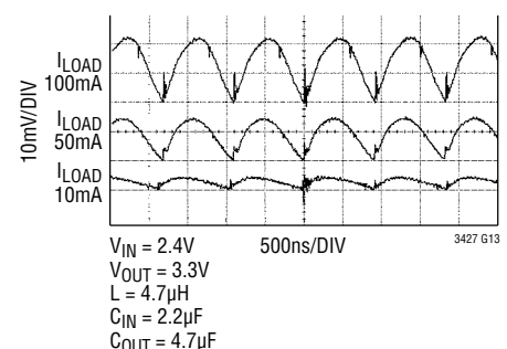
V_{OUT} Ripple, AC Coupled
