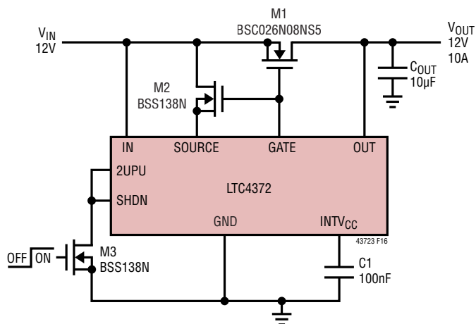
Figure 16. 12V Ideal Diode with Shutdown I_{CC} of 0.5 \mu A (Nominal)
