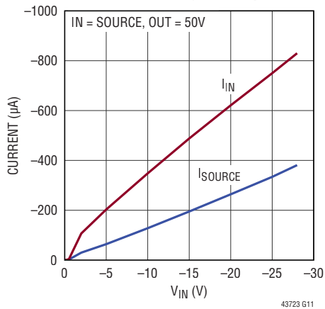
Pin Current at Negative Input
