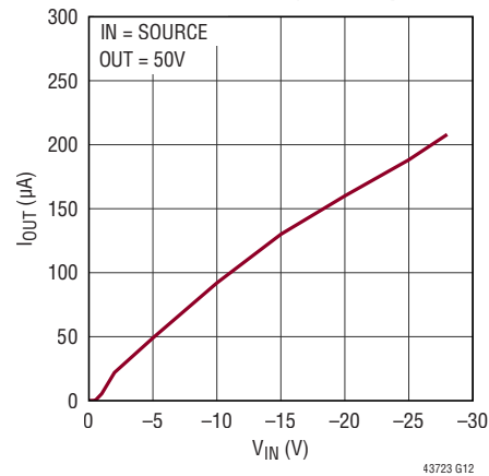
OUT Current at Negative Input
