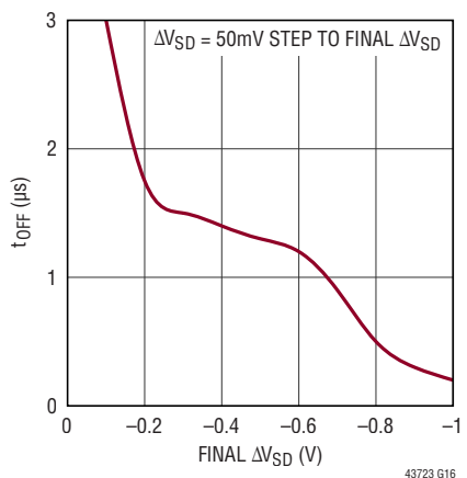
GATE Turn-Off Time vs Forward Overdrive
