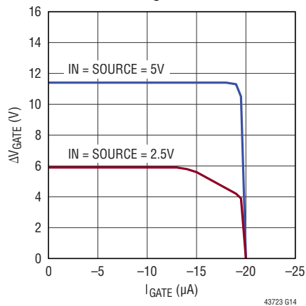
\Delta V_{\text{GATE}} (Average) vs GATE Leakage
