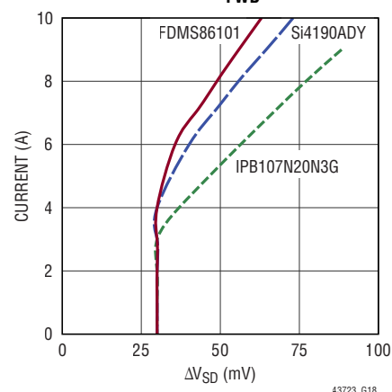
Load Current vs V_{\text{FWD}}
