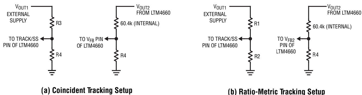
Figure 4. Setup for Coincident and Ratio-Metric Tracking
