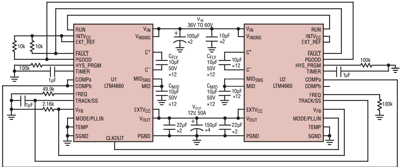
Current Sharing
