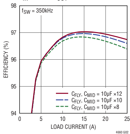
Efficiency vs Output Current V_{IN} = 54V , V_{OUT} = 12V
