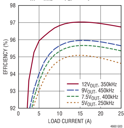
Efficiency for 54V_{IN} , C_{MID} = C_{FLY} = 10µF \times 12
