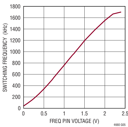
Switching Frequency vs FREQ
