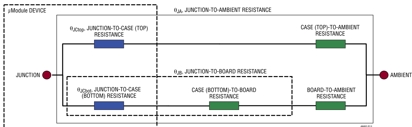
Figure 11. Graphical Representation of Thermal Coefficients, Including JEDEC51-12 Terms
