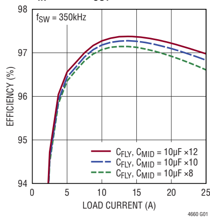
Efficiency vs Output Current V_{IN} = 48V , V_{OUT} = 12V
