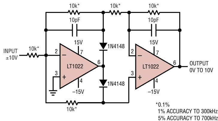
Wide Bandwidth Absolute Value Circuit
