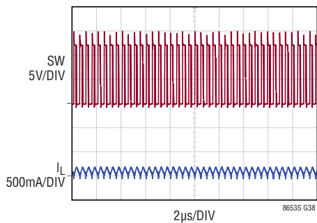
Forced Continuous Mode (FCM)
