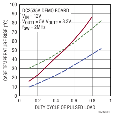
Case Temperature Rise
