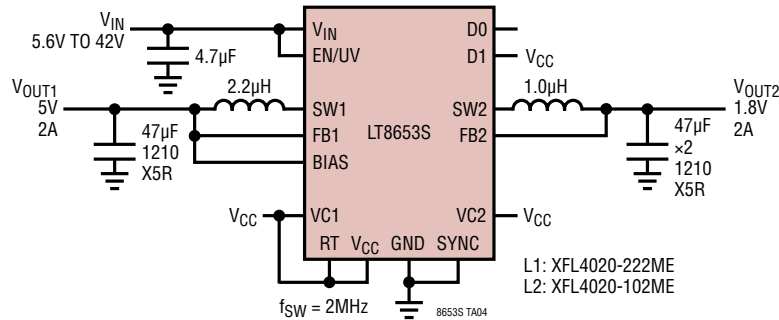
5V, 1.8V, 2MHz Step-Down Converter
