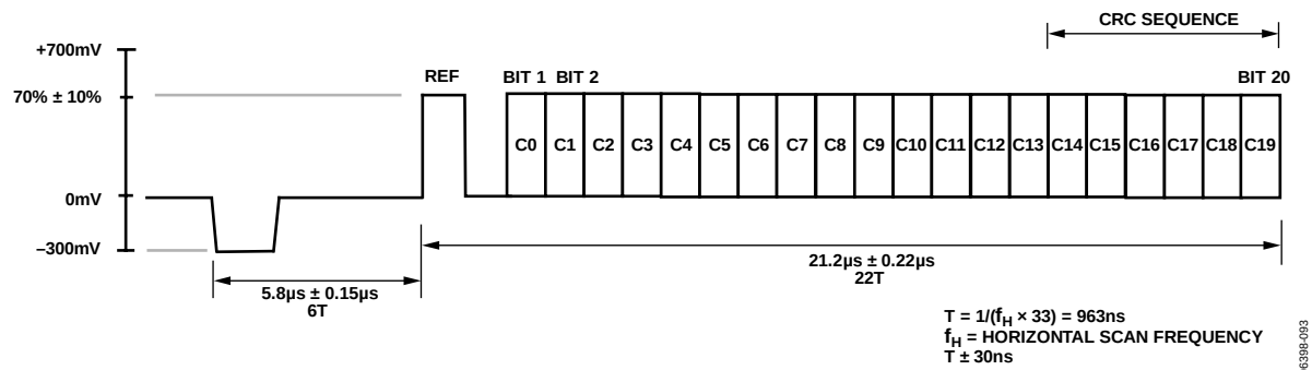
Figure 91. Enhanced Definition (525p) CGMS Waveform
