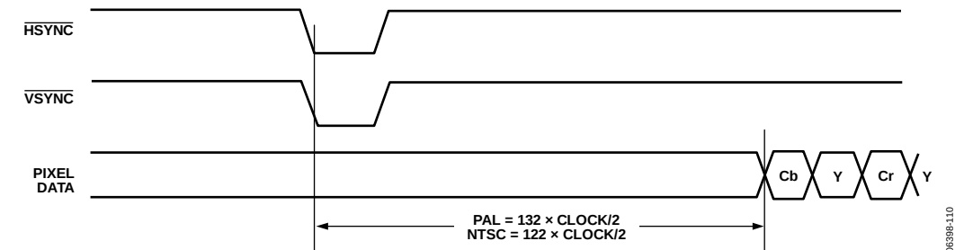
Figure 108. SD Timing Mode 2, Even-to-Odd Field Transition (Master/Slave)
