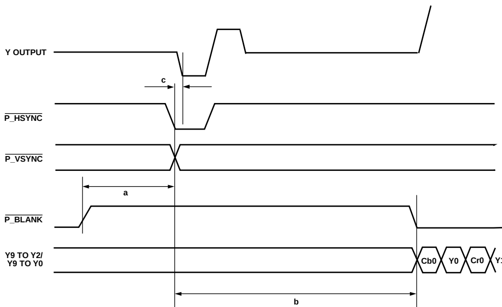
Figure 16. HD-SDR, 16-/20-Bit, 4:2:2 YCrCb ( \overline{\text{HSYNC}} / \overline{\text{VSYNC}} ) Input Timing Diagram
