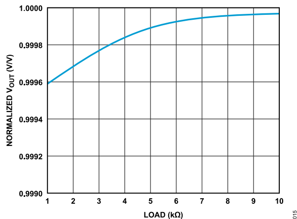
Figure 15. Normalized V_{OUT} vs. Load
