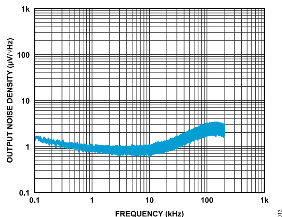
Figure 13. Output Noise Density vs. Frequency
