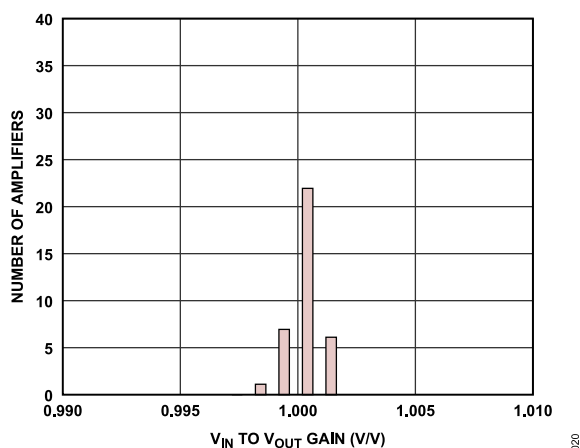
Figure 20. V_{IN} to V_{OUT} Gain Distribution at -40°C
