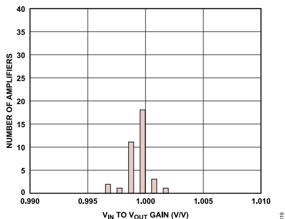
Figure 19. V_{IN} to V_{OUT} Gain Distribution at 125°C
