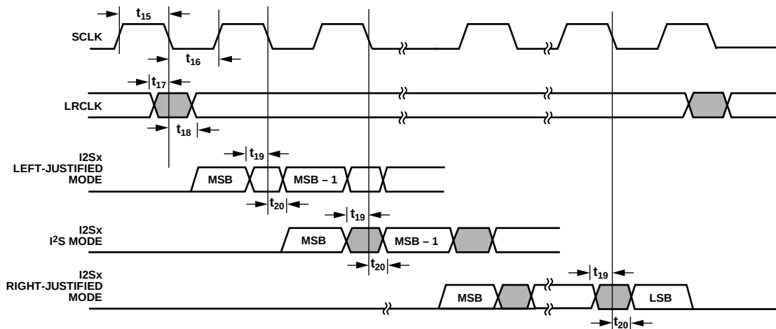
Figure 6. I²S Timing
