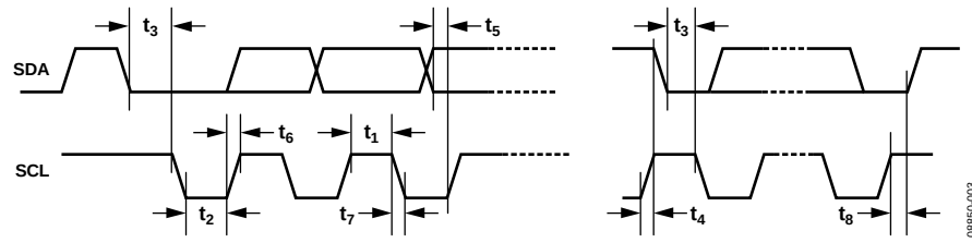
Figure 3. I²C Timing
