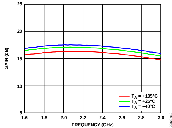
Figure 19. Gain vs. Frequency at Various Temperatures, 1.6 GHz to 3.0 GHz
