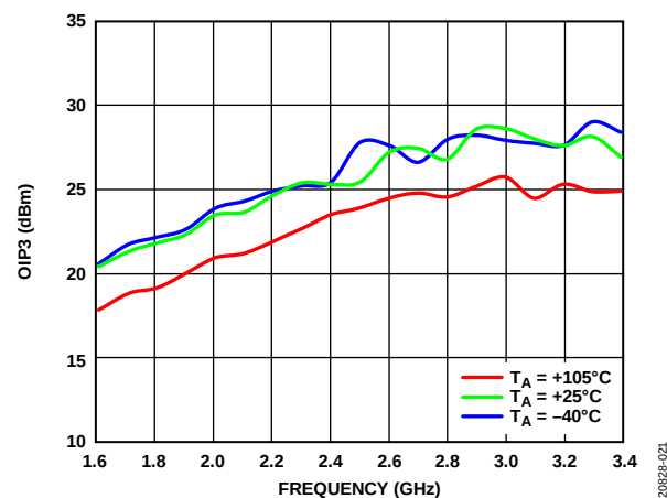
Figure 21. OIP3 vs. Frequency at -8 dBm Output Tone Power
