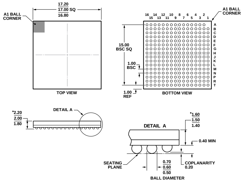
Figure 20. 255-Ball Chip-Scale Package Ball Grid Array [CSP_BGA] (BC-255-1) Dimensions shown in millimeters
