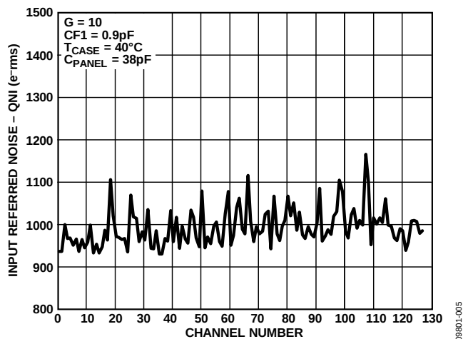
Figure 5. Input Referred Noise (QNI) vs. Channel, C_{PANEL} = 38pF , T_{CASE} = 40^{\circ}C
