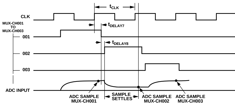
Figure 18. Input Register Timing Diagram
