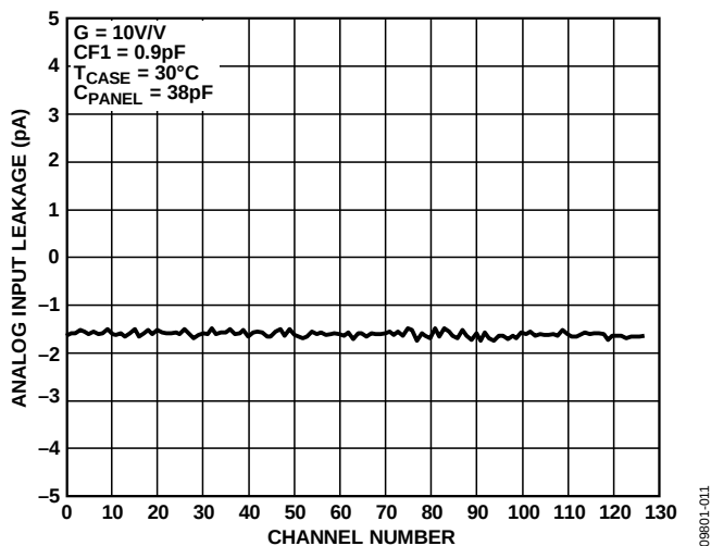
Figure 11. Input Leakage vs. Channel
