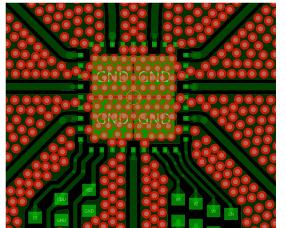
Figure 29. PCB Routs
