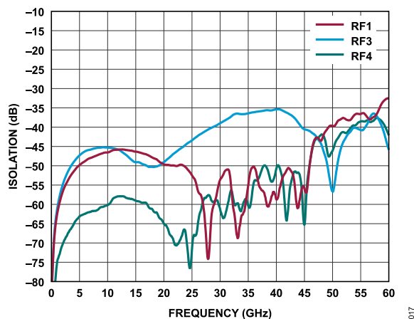
Figure 17. RF2 to RFx Isolation vs. Frequency, RF2 Selected
