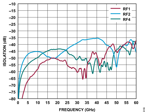
Figure 18. RF3 to RFx Isolation vs. Frequency, RF3 Selected
