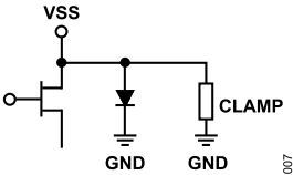
Figure 7. VSS Interface Schematic
