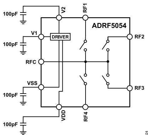
Figure 24. Recommended Schematic
