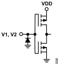
Figure 6. V1, V2 Pin Interface Schematic
