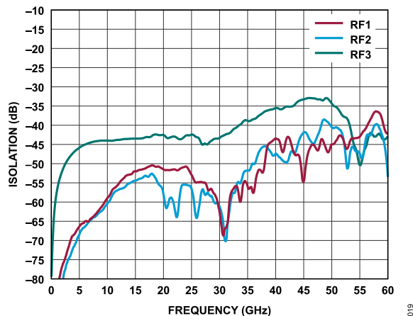
Figure 19. RF4 to RFx Isolation vs. Frequency, RF4 Selected
