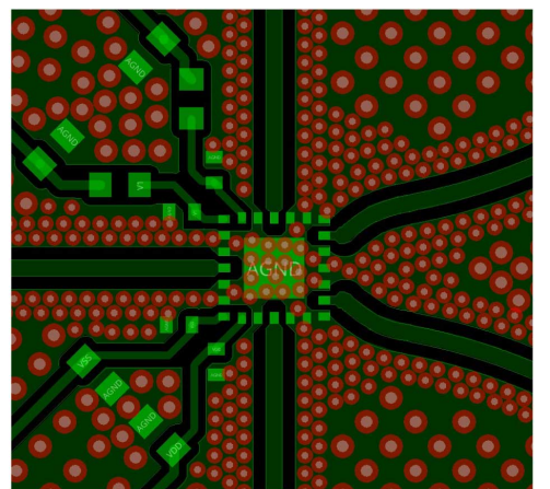
Figure 26. PCB Layout
