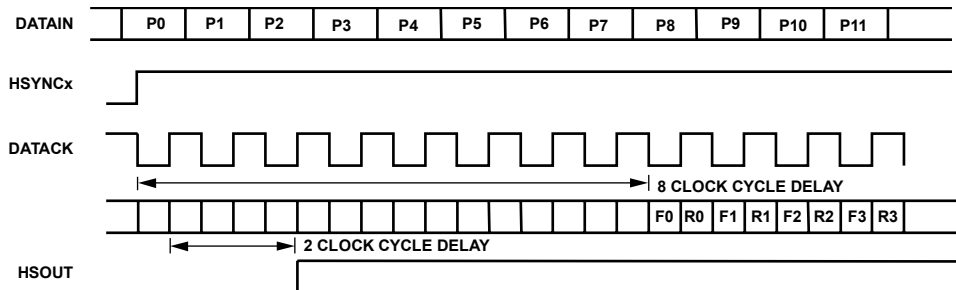
Figure 15. 4:2:2 Timing Mode
