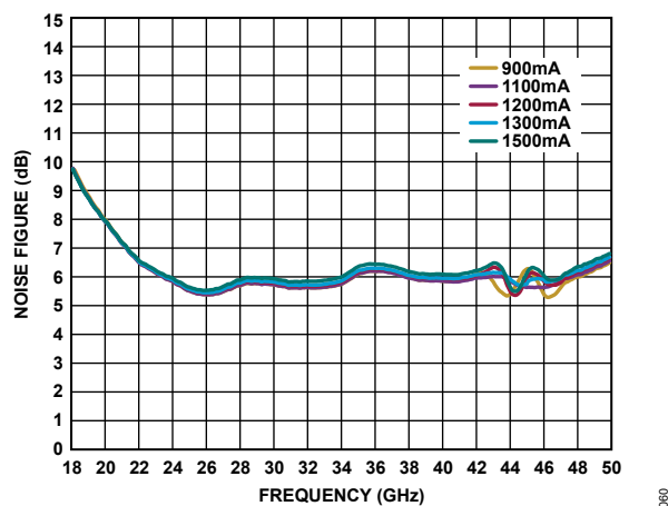
Figure 61. Noise Figure vs. Frequency for Various Supply Currents, V_{DD} = 3\text{ V}
