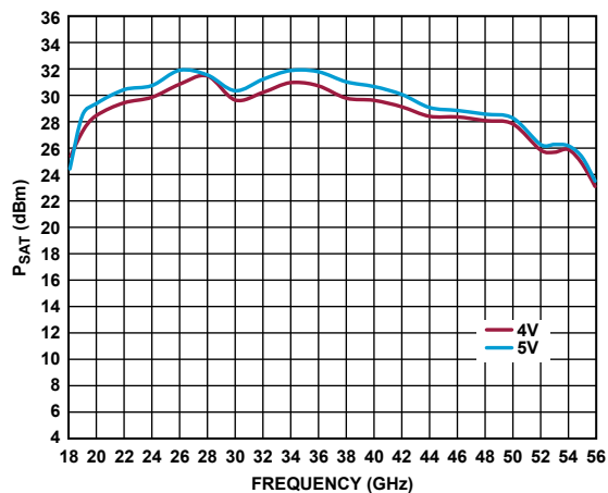
Figure 31. P_{SAT} vs. Frequency for Various Voltages, I_{DQ} = 1500 mA
