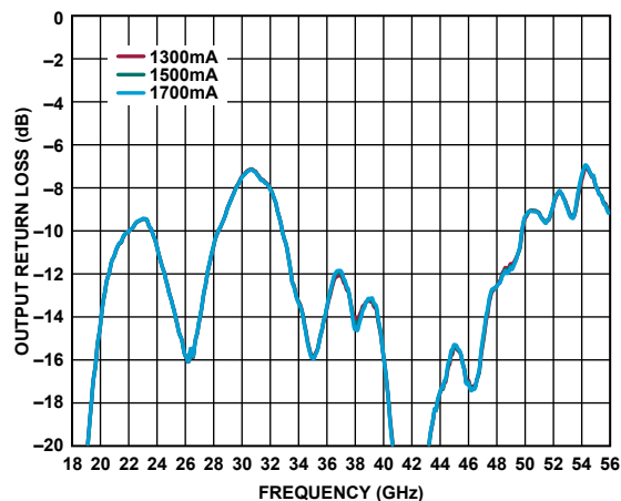
Figure 20. Output Return Loss vs. Frequency for Various Supply Currents, V_{DD} = 5\text{ V}
