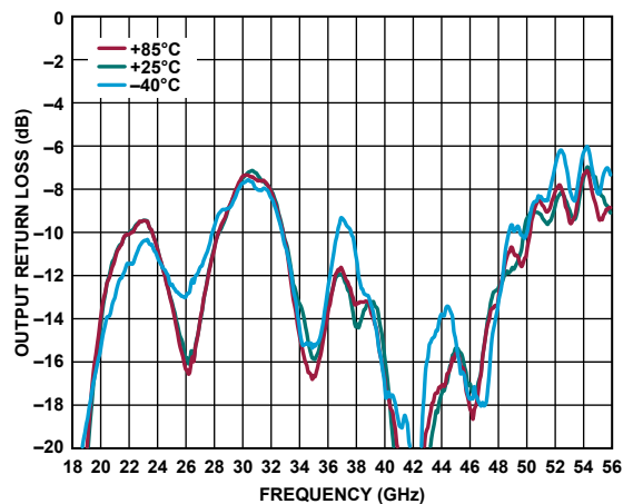
Figure 19. Output Return Loss vs. Frequency for Various Temperatures, V_{DD} = 5\text{ V} , I_{DQ} = 1500\text{ mA}
