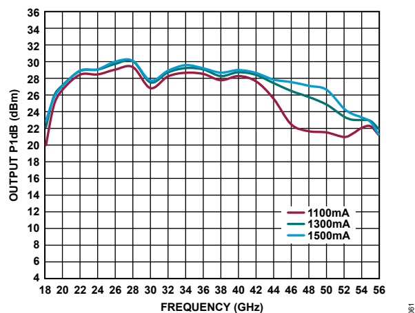
Figure 62. Output P1dB vs. Frequency for Various Supply Currents, V_{DD} = 4\text{ V}
