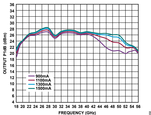
Figure 59. Output P1dB vs. Frequency for Various Supply Currents, V_{DD} = 3\text{ V}
