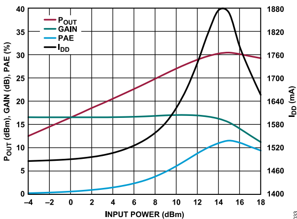
Figure 33. P_{OUT} , Gain, PAE, and Drain Current with RF Applied ( I_{DD} ) vs. Input Power, 22 GHz, V_{DD} = 5 V, I_{DQ} = 1500 mA
