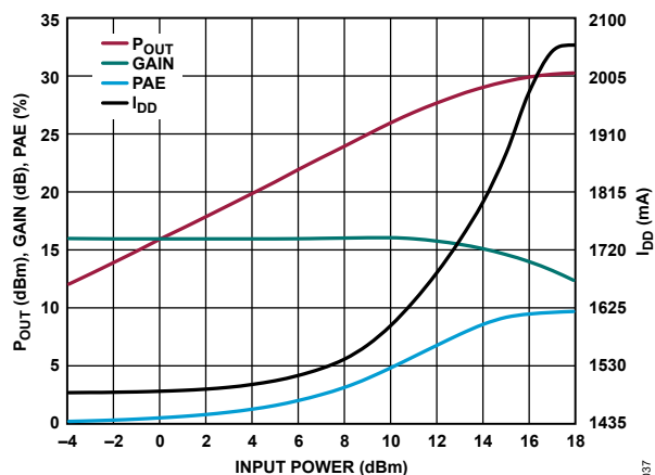
Figure 37. P_{OUT} , Gain, PAE, and I_{DD} vs. Input Power, 30 GHz, V_{DD} = 5 V, I_{DQ} = 1500 mA
