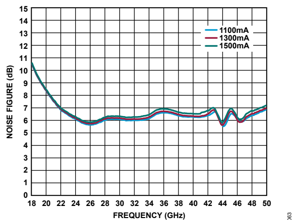
Figure 64. Noise Figure vs. Frequency for Various Supply Currents, V_{DD} = 4\text{ V}
