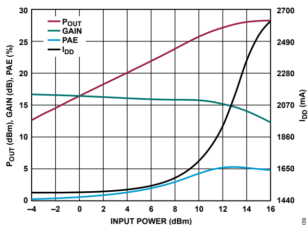
Figure 39. P_{OUT} , Gain, PAE, and I_{DD} vs. Input Power, 50 GHz, V_{DD} = 5 V, I_{DQ} = 1500 mA
