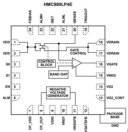
Figure 74. Functional Diagram of HMC980LP4E
