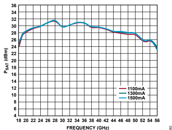
Figure 63. P_{SAT} vs. Frequency for Various Supply Currents, V_{DD} = 4\text{ V}
