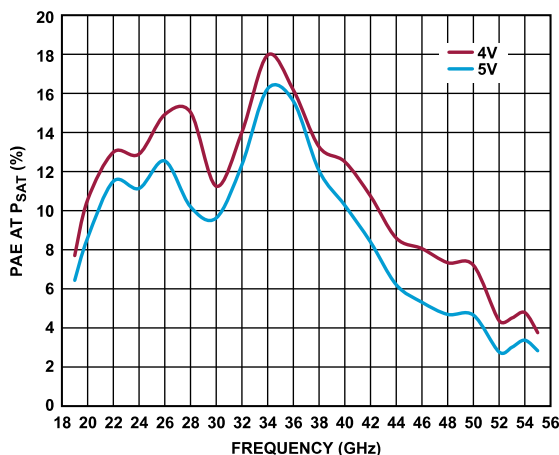
Figure 32. PAE at P_{SAT} vs. Frequency for Various Supply Voltages, I_{DQ} = 1500 mA
