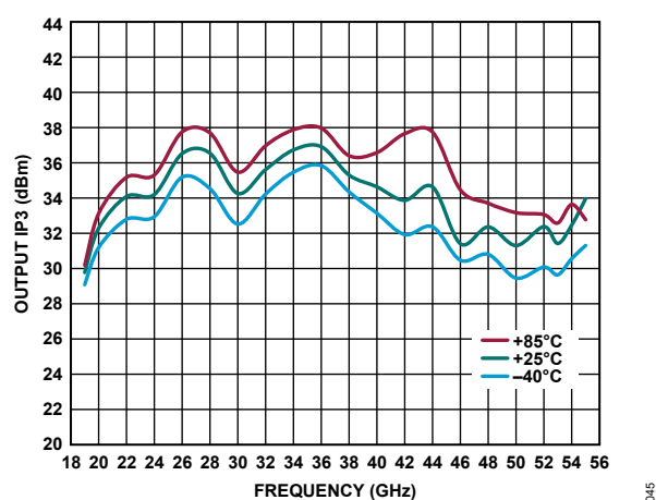
Figure 45. Output IP3 vs. Frequency for Various Temperatures, P_{OUT} per Tone = 14 dBm, V_{DD} = 5\text{ V} , I_{DQ} = 1700\text{ mA}
