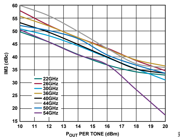
Figure 49. IM3 vs. P_{OUT} per Tone for Various Frequencies, V_{DD} = 4\text{ V} , I_{DQ} = 1500\text{ mA}
