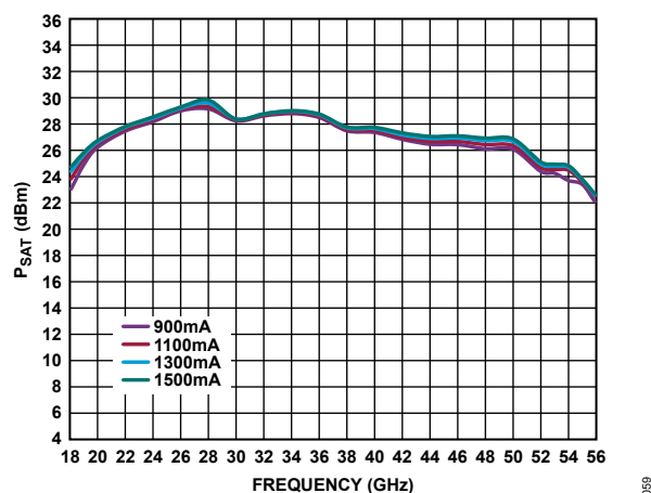
Figure 60. P_{SAT} vs. Frequency for Various Supply Currents, V_{DD} = 3\text{ V}
