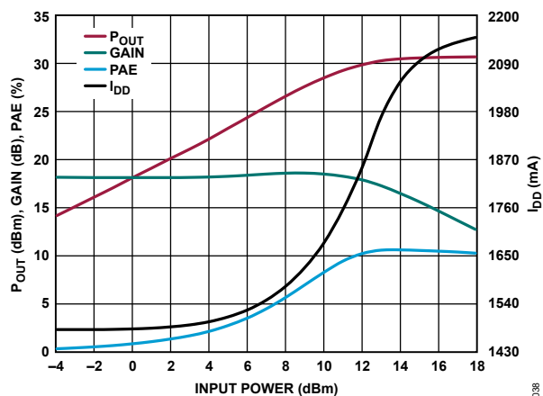
Figure 38. P_{OUT} , Gain, PAE, and I_{DD} vs. Input Power, 40 GHz, V_{DD} = 5 V, I_{DQ} = 1500 mA
