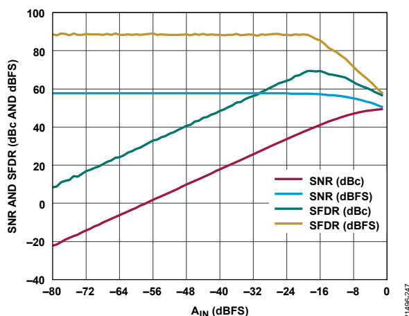
Figure 47. Single-Tone SFDR and SNR vs. A_{IN} at f_{IN} = 4.5 GHz
