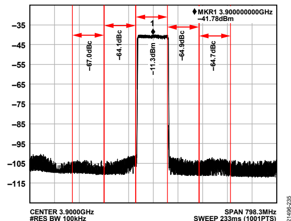
Figure 35. ACLR Performance for 100 MHz 5G Test Vector at f_{OUT} = 3.9 GHz and f_{DAC} = 11.898 GSPS, Test Vector Peak to RMS = 11.7 dB with -1 dBFS Backoff (Mode 9C), Channel Interpolation 3 \times , Main Interpolation 8 \times
