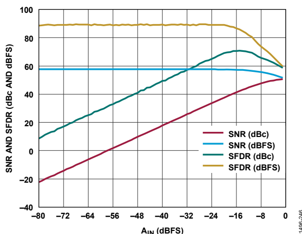
Figure 46. Single-Tone SFDR and SNR vs. A_{IN} at f_{IN} = 3.6 GHz
