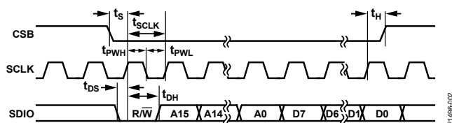
Figure 2. Timing Diagram for 3-Wire Write Operation
