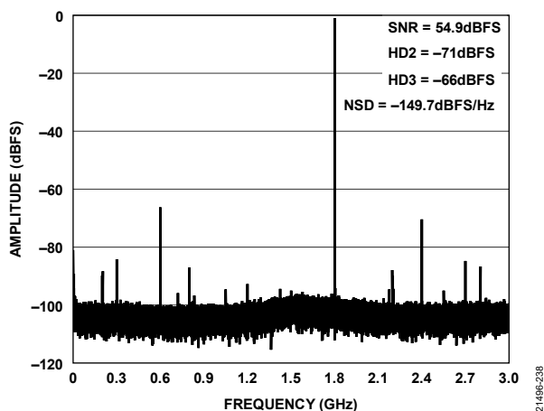
Figure 38. Single-Tone FFT at f_{IN} = 1.8 GHz
