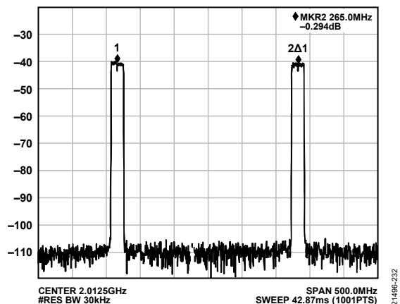
Figure 32. Dual Band Wideband Plot for Two 20 MHz LTE Carriers at f_{OUT} = 1.88 GHz and f_{OUT} = 2.145 GHz (3GPP Bands, B1 and B3, Respectively), at f_{DAC} = 11.796 GSPS, Test Vector PAR = 7.7 dB with -1 dBFS Backoff, Channel Interpolation 3 \times , Main Interpolation 8 \times , Mode 9C
