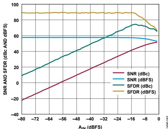
Figure 45. Single-Tone SFDR and SNR vs. A_{IN} at f_{IN} = 2.7 GHz
