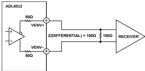
Figure 61. Simplified ADL6012 Output Interface
