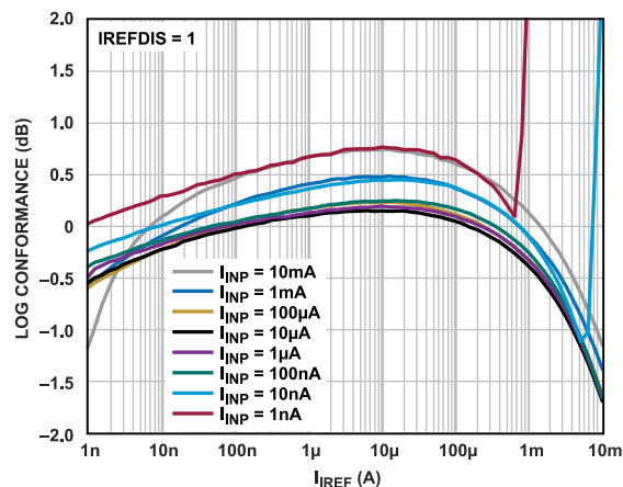
Figure 13. Log Conformance Error vs. I_{REF} at Various I_{INP} Value in Decade Steps
