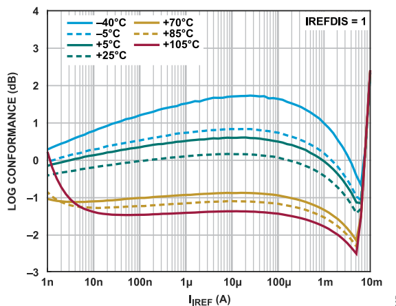
Figure 8. Log Conformance Error vs. I_{REF} at Various Temperatures for I_{INP} = 10\text{ nA} , Normalized to 25^\circ\text{C}
