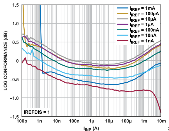
Figure 9. Log Conformance Error vs. I_{INP} at Various I_{REF} Values in Decade Steps
