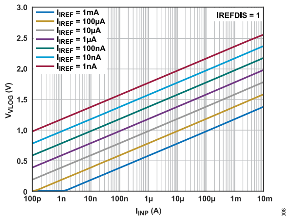
Figure 6. V_{LOG} vs. I_{INP} at Various I_{REF} Values in Decade Steps
