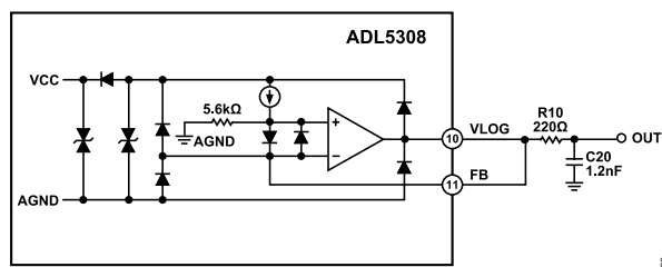
Figure 40. Simplified Schematic of the Low-Pass Filter Network at the VLOG
