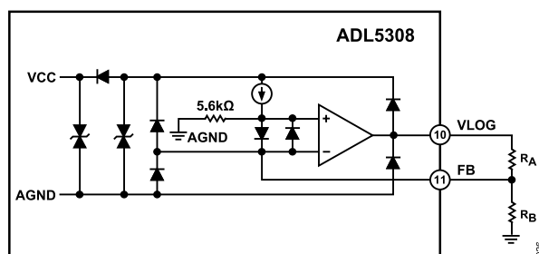
Figure 39. Simplified Schematic of VLOG and FB Interface
