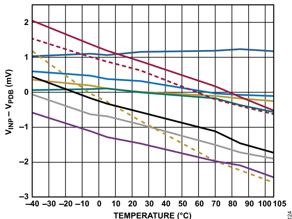
Figure 12. Offset Voltage V_{INP} - V_{PDB} at 10 nA vs. Temperature Over 10 Samples
