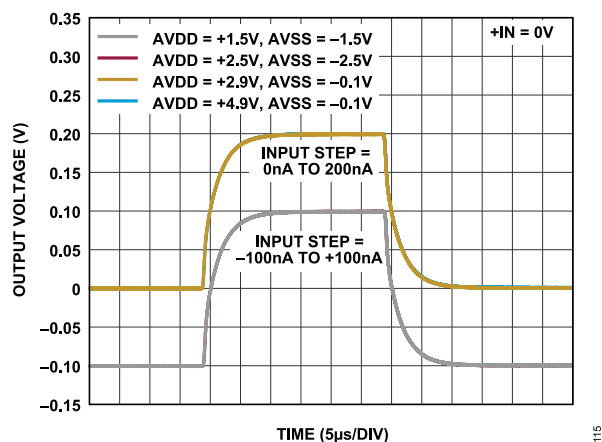
Figure 69. Small-Signal Step Response at Various Supplies, C_{IN} = 10 pF, R_F = 1 M \Omega
