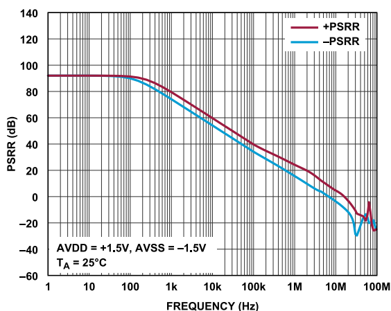
Figure 59. PSRR vs. Frequency, AVDD = +1.5\text{ V} , AVSS = -1.5\text{ V}
