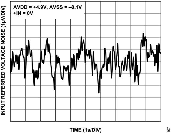
Figure 51. 0.1 Hz to 10 Hz Voltage Noise, AVDD = +4.9 V, AVSS = -0.1 V
