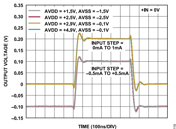
Figure 71. Small-Signal Step Response at Various Supplies, C_{IN} = 10 pF, R_F = 200 \Omega
