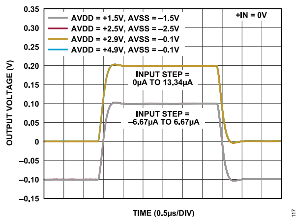
Figure 70. Small-Signal Step Response at Various Supplies, C_{IN} = 10 pF, R_F = 15 k \Omega , C_{F,EXT} = 5.6 pF
