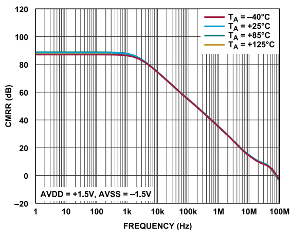
Figure 58. CMRR vs. Frequency over Various Temperatures, AVDD = 1.5\text{ V} , AVSS = -1.5\text{ V}
