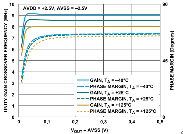
Figure 43. Unity Gain Crossover Frequency and Phase Margin vs. V_{OUT} - AVSS , No Load, AVDD = +2.5\text{ V} , AVSS = -2.5\text{ V}
