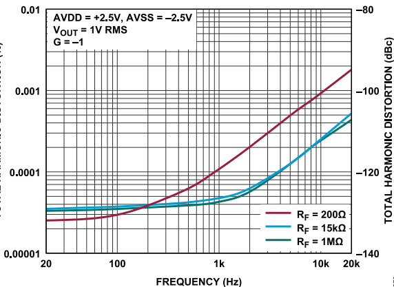
Figure 53. Total Harmonic Distortion vs. Frequency, AVDD = +2.5 V, AVSS = -2.5 V
