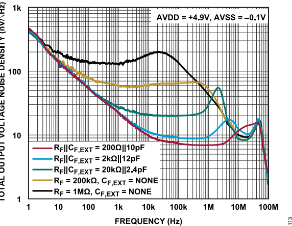
Figure 52. Total Output Voltage Noise Density vs. Frequency, AVDD = +4.9 V, AVSS = -0.1 V
