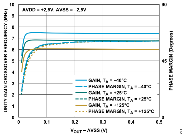
Figure 44. Unity Gain Crossover Frequency and Phase Margin vs. V_{OUT} - AVSS , Load = Low-Pass Output Filter ( R_{EXT} = 25\ \Omega , C_{EXT} = 1\text{ nF} ), AVDD = +2.5\text{ V} , AVSS = -2.5\text{ V}
