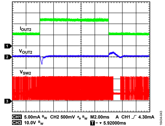
Figure 43. Buck Regulator Load Transient Response, V_{OUT1} = 21V , V_{OUT2} = 5.15V , I_{OUT2} = 0.3mA to 7mA Step, T_A = 25^\circ C
