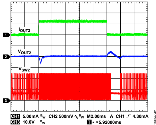
Figure 40. Buck Regulator Load Transient Response, V_{OUT1} = 24V , V_{OUT2} = 5.15V , I_{OUT2} = 0.3mA to 7mA Step, T_A = 25^\circ C
