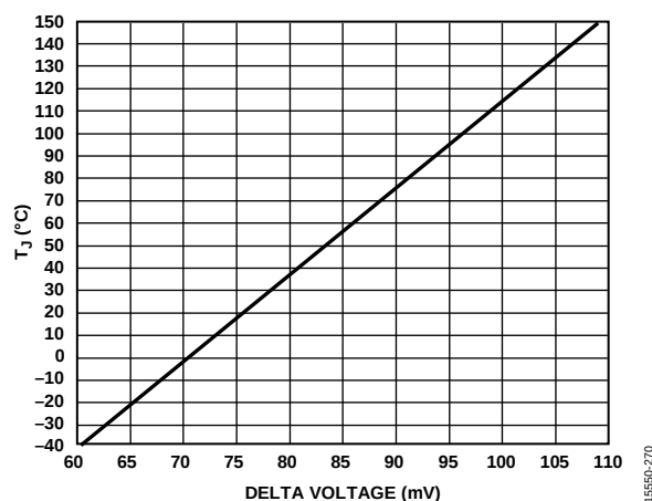
Figure 100. Junction Temperature vs. \Delta V (mV)
